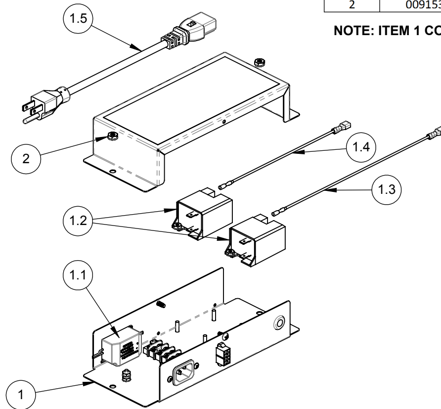
DOUBLE SIDE BURNER ELECTRICAL BOX SHOWN FOR REFERENCE
