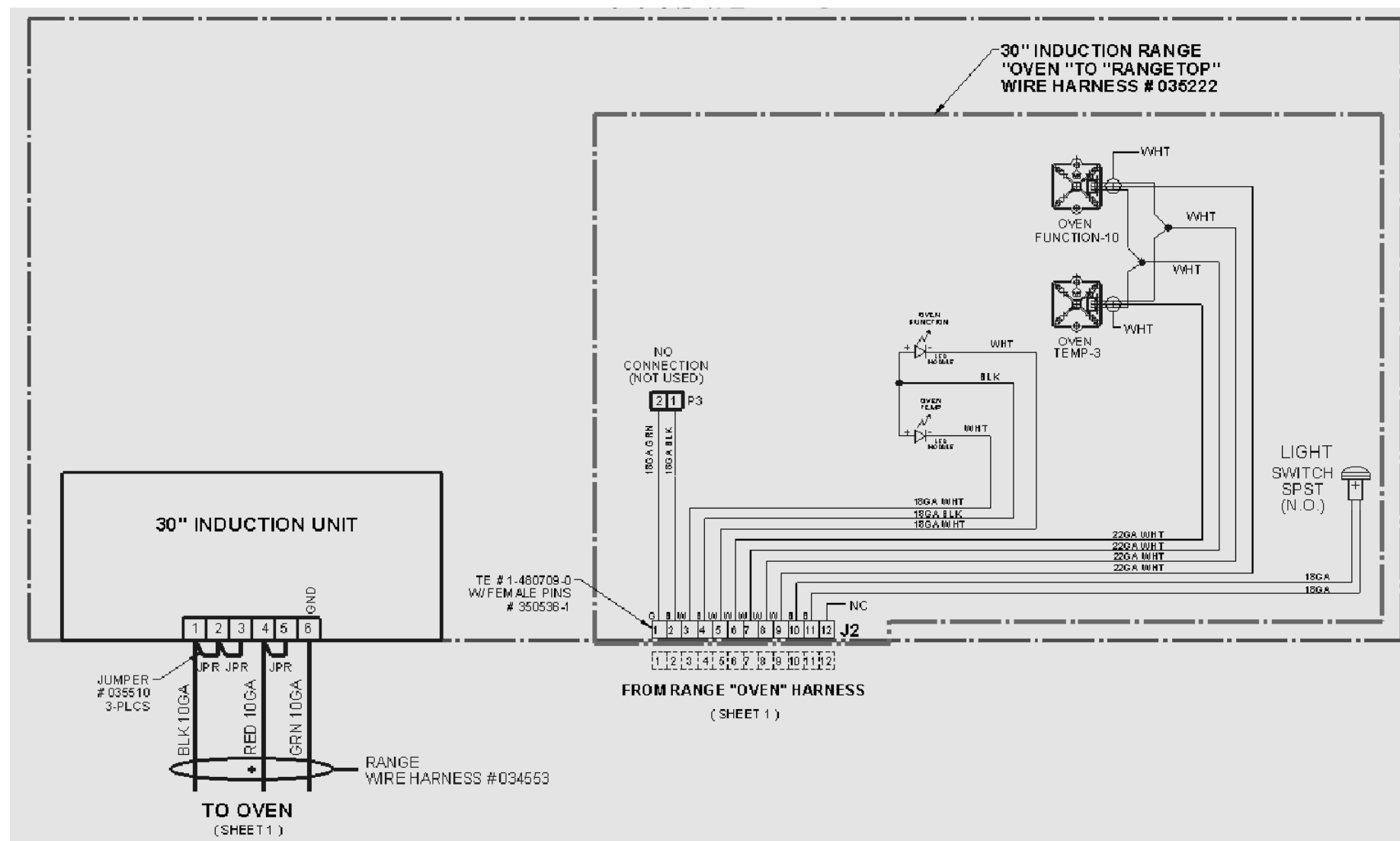
WIRING DIAGRAM, 30 INDUCTION RANGE 034556
