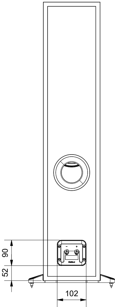
BACK
