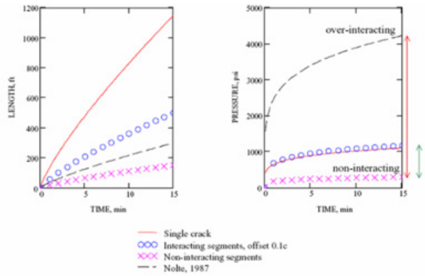
Figure 13 > Fracture length and treating pressures for 29 interacting parallel fractures.
