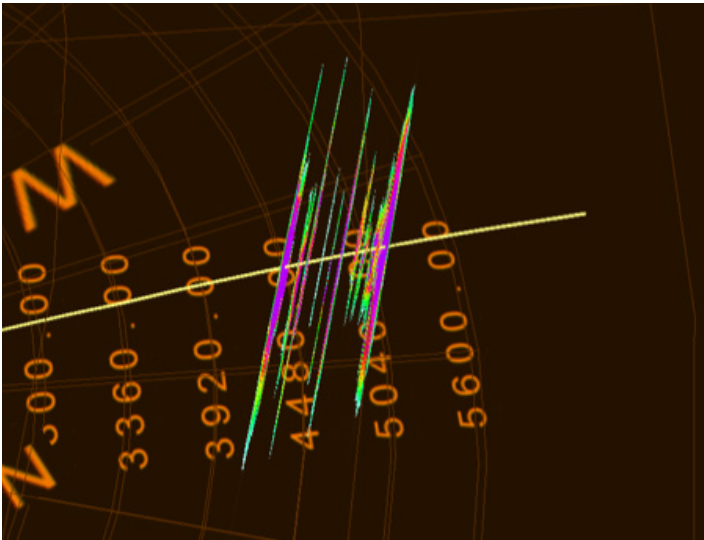
Figure 9 > GOHFER output for non-orthogonal interfering fractures. Plan view looking down on the two stages (10 total clusters).
