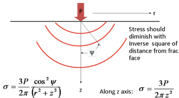
Figure 2 > Boussinesq (1885) solution for stress distribution in a linear-elastic half-space acted upon by an externally applied load.
