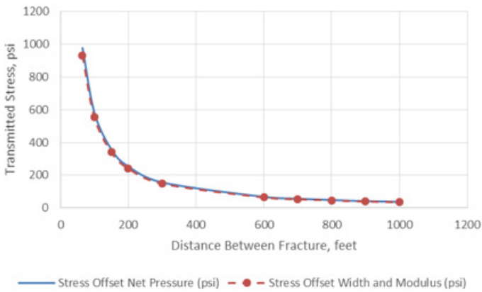
Figure 6 > Comparison of the stress shadow for Eq. 1 and Eq. 2 with \nu = 1.2 .
