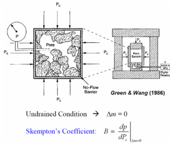
Figure 4 > Definition of Skempton's coefficient B for undrained compaction.
