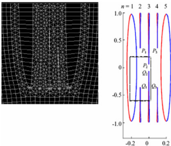
Figure 12 > Stabilized fracture profiles for five parallel interacting fractures.
