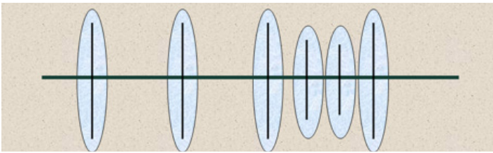
Figure 1 > Illustration of “stress shadowing” for multiple fractures. The heavy line represents the horizontal wellbore, the vertical lines represent the hydraulic fractures, and the blue ellipses represent the stress-shadowed regions.
