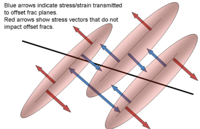
Figure 8 > Illustration of stress shadow propagation for non-orthogonal and asymmetric fractures.
