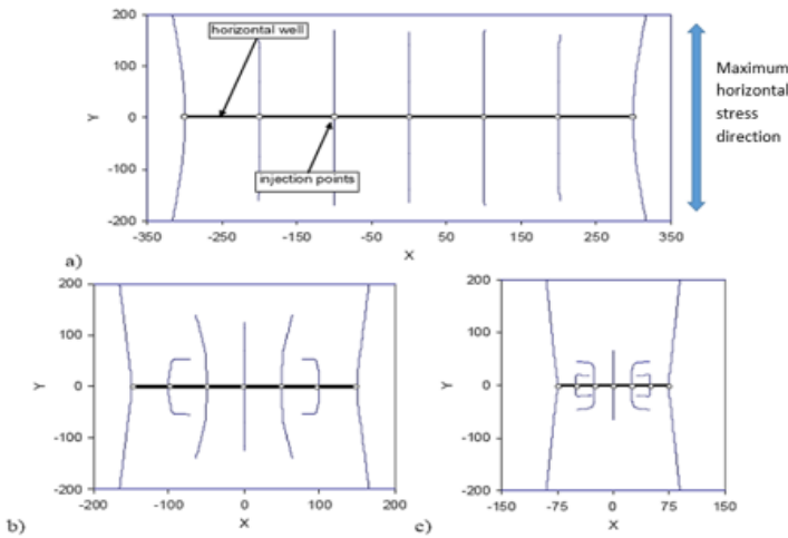
Figure 11 > Illustration of curving fractures in an isotropic linear-elastic 2D model (Olson, 2008).
