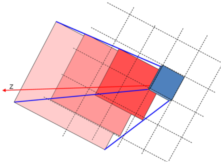
Figure 7 > Illustration of the stress shadow from a single fracture face cell to offset planes.
