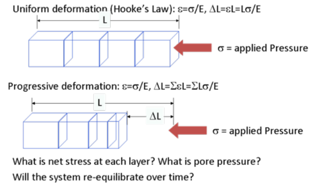
Figure 3 > Concept of progressive (lower figure) versus uniform (upper figure) deformation for unconventional reservoir stimulation.
