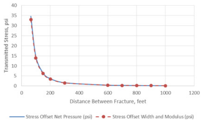
Figure 5 > Comparison of the stress shadow for Eq. 1 and Eq. 2 with t = 2 .
