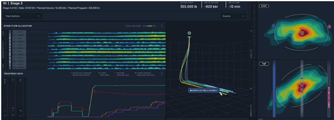
The SmartFleet system provides real-time visualization of fracture measurements, cluster uniformity and well interactions.
