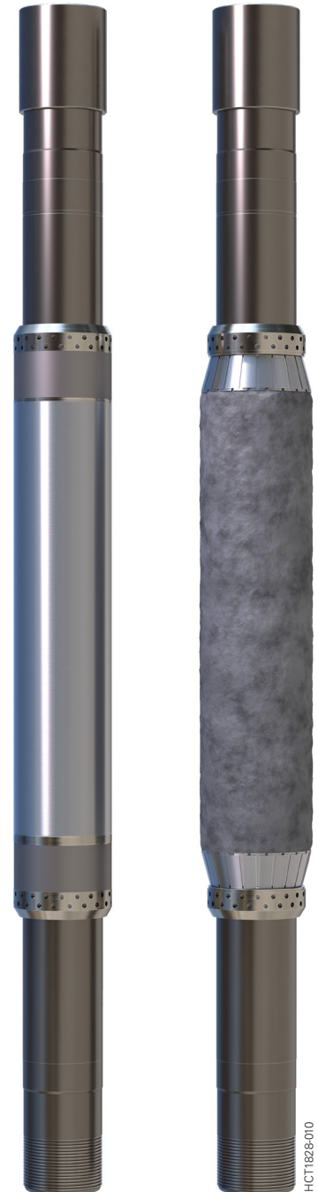
The Ovidius® expanding isolation system transforms from an engineered metal alloy into a rock-like material when it reacts with downhole fluids.
