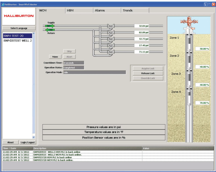
Well control module (WCM) screen
