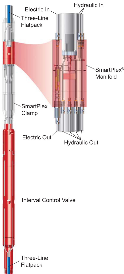
Control module with clamp assembly
