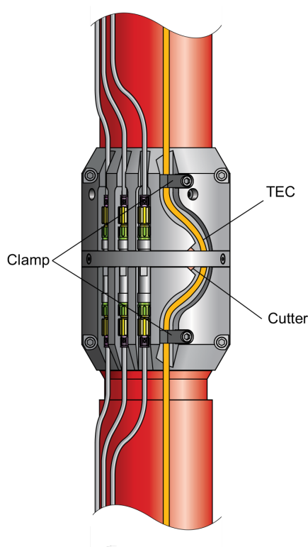
Control line cut sub (CLCS)
