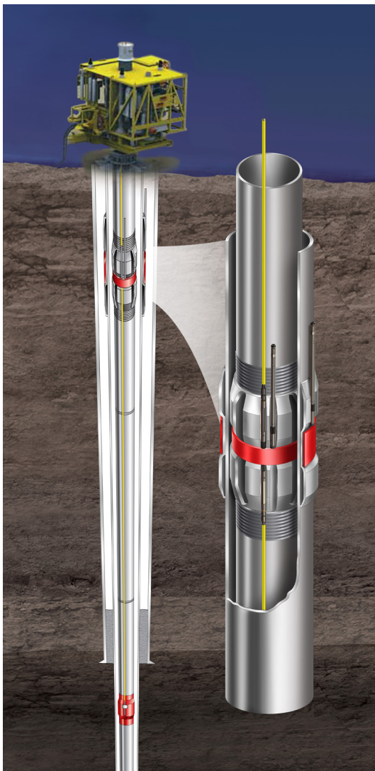
DataSphere® LinX® B-Annulus pressure/ temperature (P/T) monitoring system
