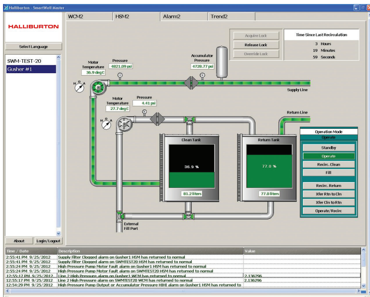
Hydraulic supply module (HSM) screen
