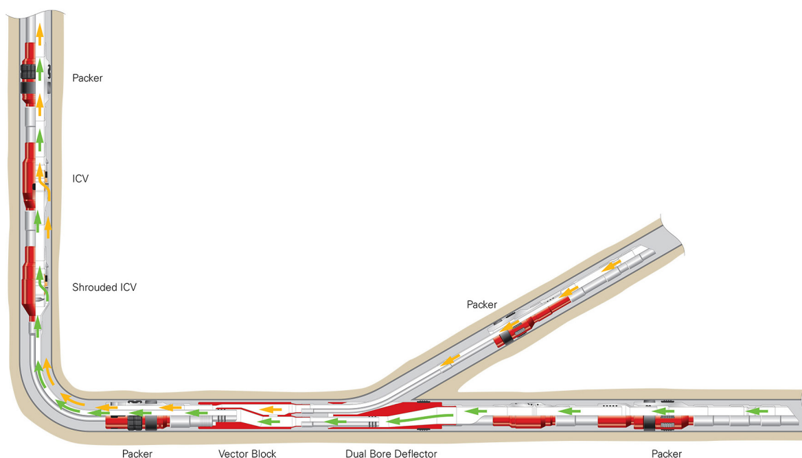
Multilateral Pressure-Isolated Level 5 with Intelligent Interface
