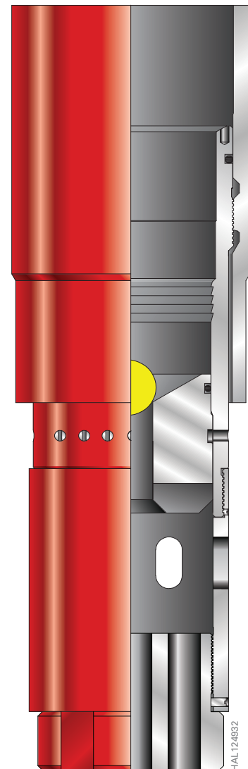
Landing Collar Latch Type with Catcher Sub
