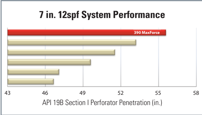
390 MaxForce is the industry's deepest-penetrating charge for 4 5/8-in. 5spf and 7-in. 12spf perforating system.
