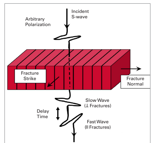
Shear-Wave Splitting
