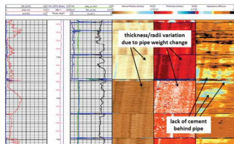
Sample CAST-M / CBL-M / MFC Casing Inspection and Cement Evaluation Log in 4-½-in. tubing, depicting a change in pipe weight
