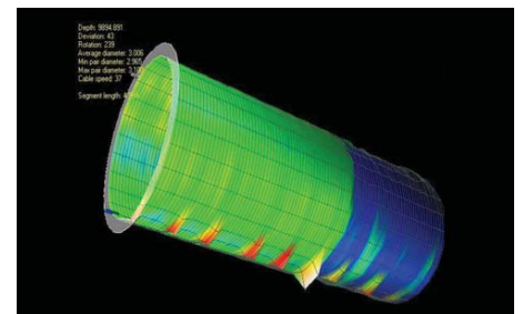
Sample 3D interactive mapping of an orifice detected in a tubular. The MFC’s high acquisition rate can provide detailed imaging to help discern minute changes in casing.
