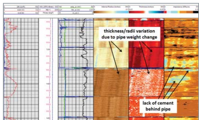
Sample CAST-M / CBL-M / MFC Casing Inspection and Cement Evaluation Log in 4-1/2-in. tubing, depicting a change in pipe weight
