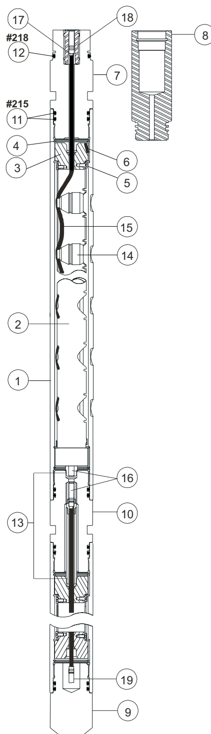
1 9/16-in. 4-spf 0° Scalloped System
