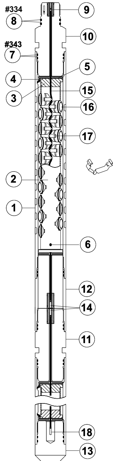
4 5/8-in. 11-spf 140°/160° Lowside VannGun™ System
