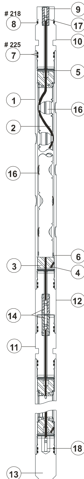
2 1/2 in. 4-spf 180° VannGun™ System
