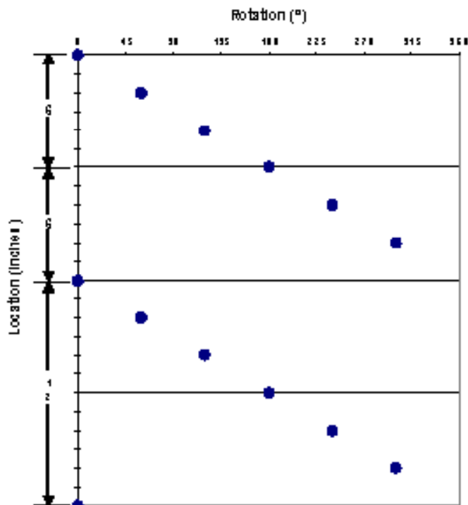
Shot Pattern for 2-in. 6-spf 60° Phasing
