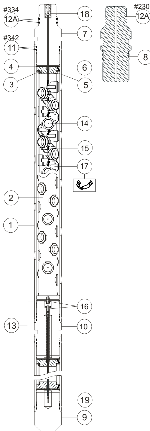
4 1/2-in. 12-spf 45°/135° Scalloped System
