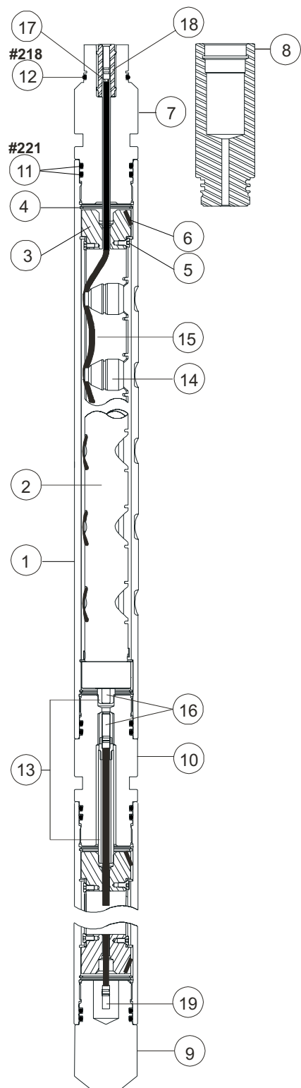
2-in. 4-spf 0° Scalloped System
