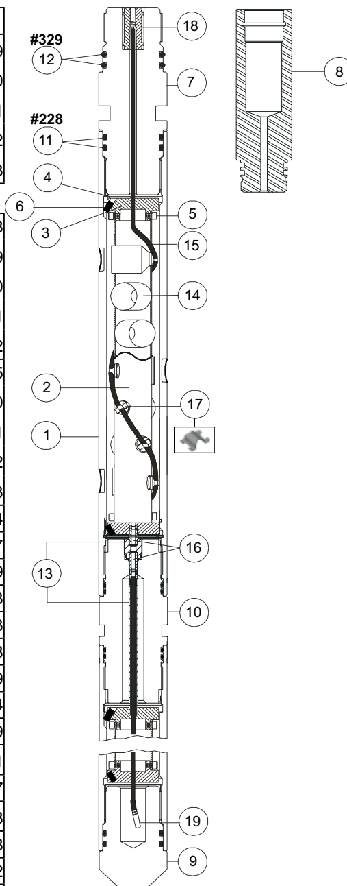
2 7/8-in. 6-spf 60° Scalloped System
