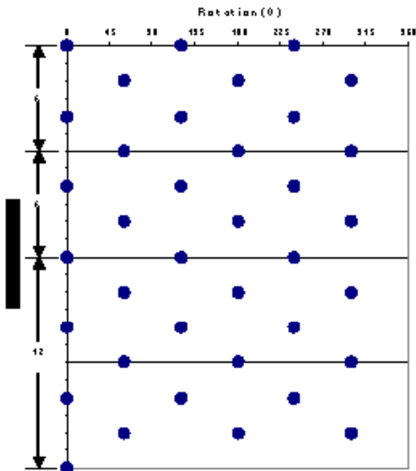
Shot Pattern for 5-in. 18-spf 60°/120° Phasing
