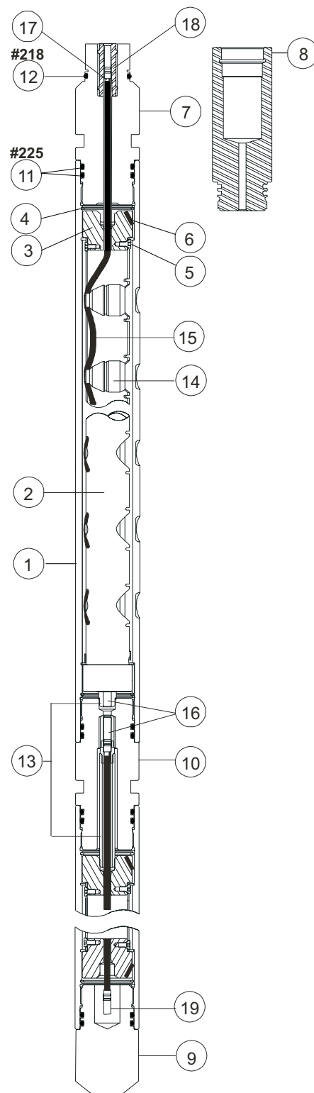
2 1/2-in. 6-spf 0° Scalloped System
