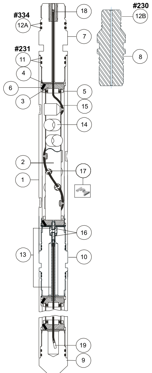
3 3/8-in. 6-spf 60° SDP Scalloped System
