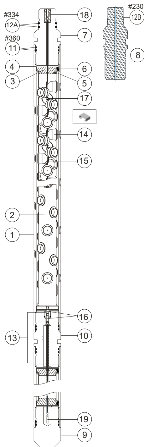
7-in. 12-spf 45°/135° BH/SH System
