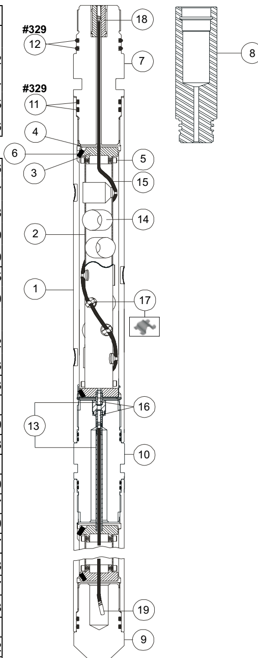
2 3/4-in. 6-spf 60° Scalloped System
