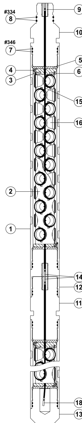
5-in. 18-spf 3/Plane SH VannGun™ System
