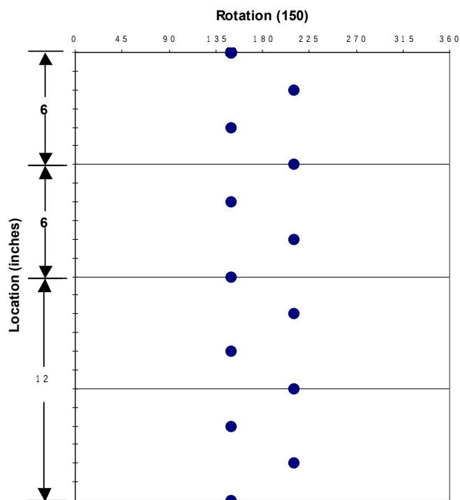
Shot Pattern for 2.75-in. 6-spf 60 Phasing
