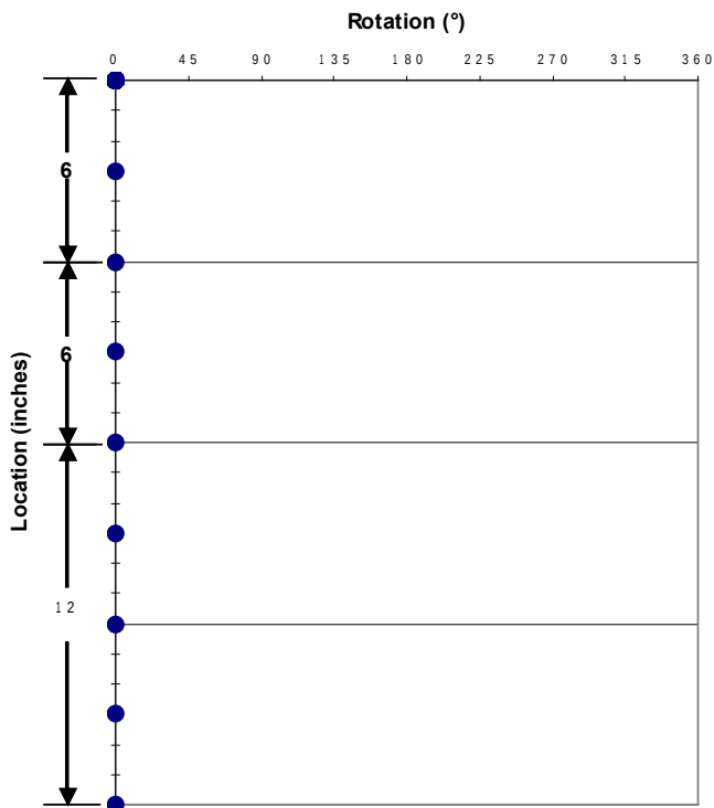
Shot Pattern for 2-in. 4-spf 0° Phasing
