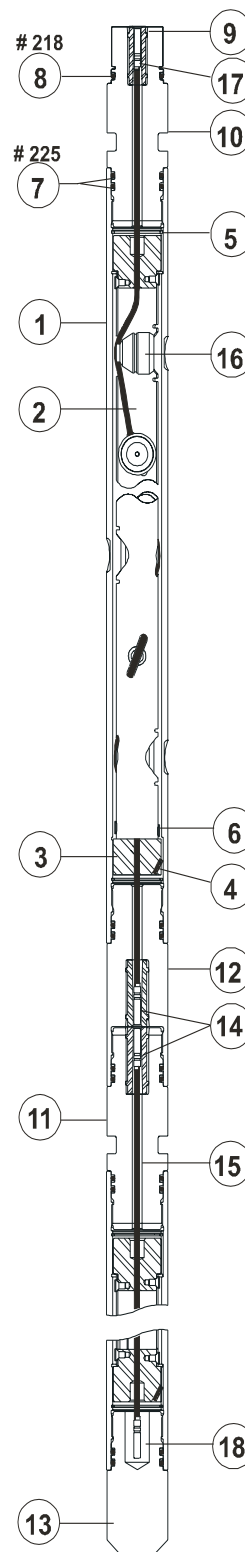
2 1/2-in. 4-spf 0° VannGun™ System
