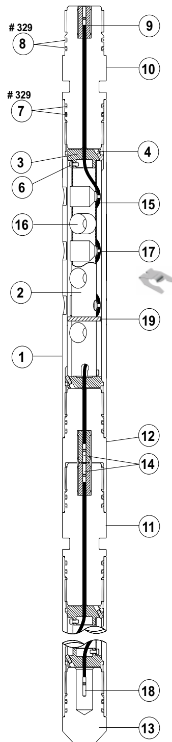
2 3/4-in. 6-spf 60° Lowside VannGun™ System
