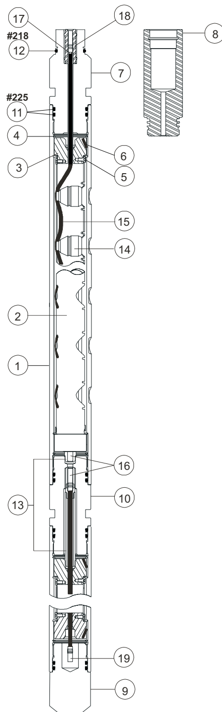
2 1/2-in. 4-spf 0° Scalloped System
