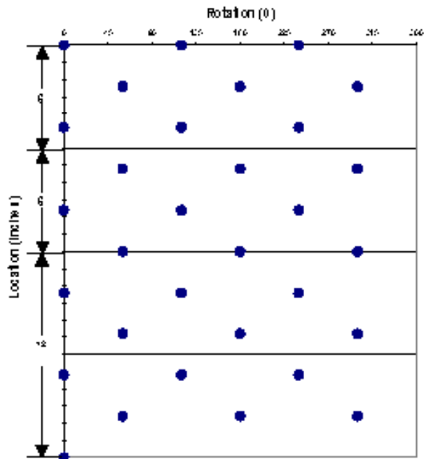
Shot Pattern for 5-in. 15-spf 60°/120° Phasing
