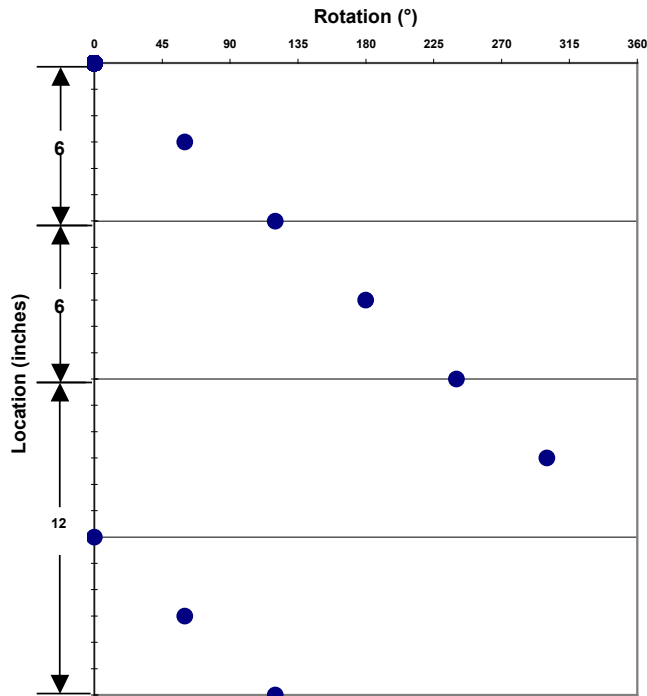
Shot Pattern for 3.37-in. 4-spf 60° Phasing
