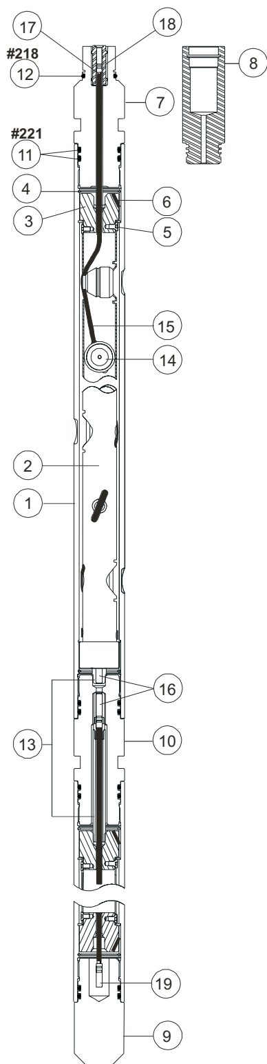
2-in. 4-spf 90° Scalloped System
