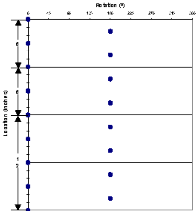
Shot Pattern for 4.625-in. 8-spf 180° Phasing
