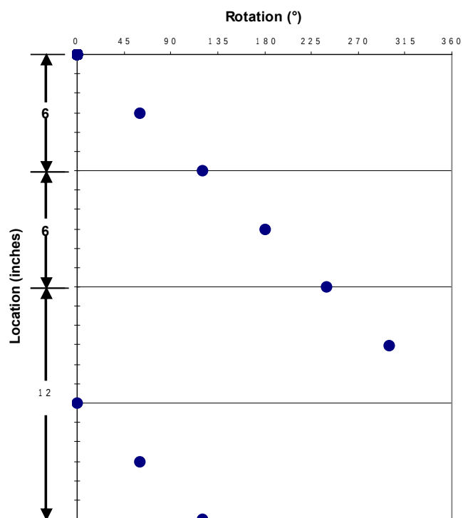
Shot Pattern for 2-in. 4-spf 60° Phasing
