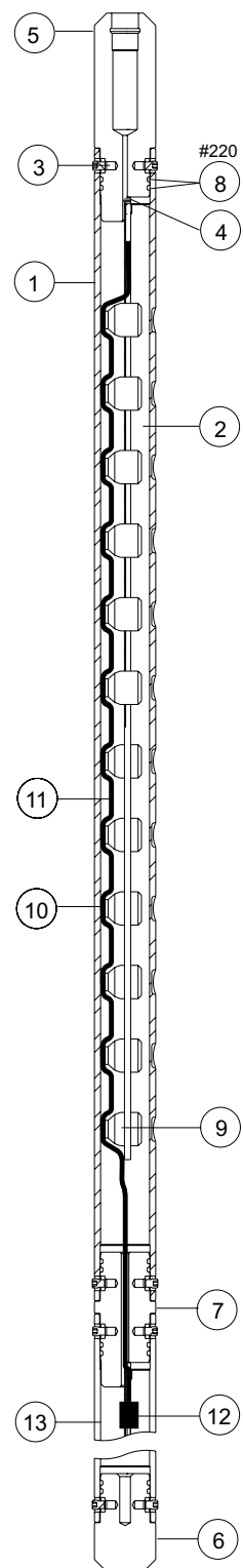
2-in. 6-spf 0° Slip-On Tubing Puncher
