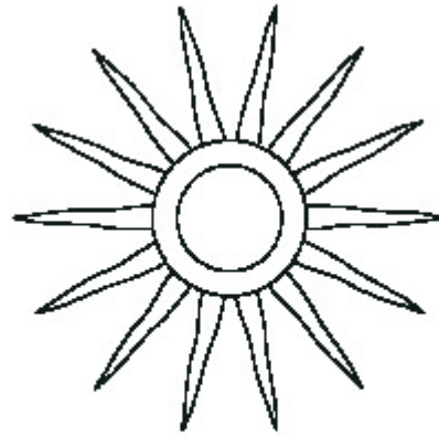
25.7°/128.5° Phasing 14 Perforation Planes
