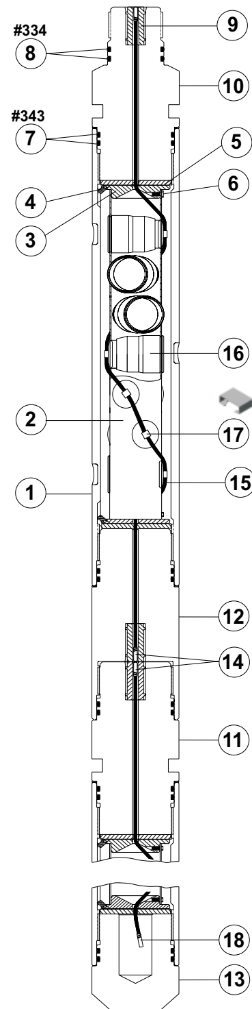
4 5/8-in. 5-spf 72° MaxForce™ VannGun™ System
