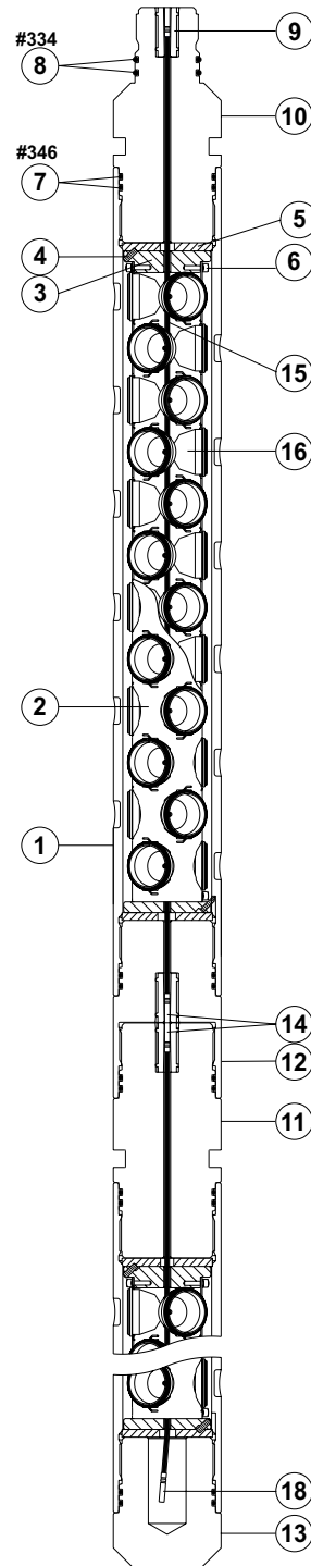
5-in. 15-spf 3/Plane SH VannGun™ System
