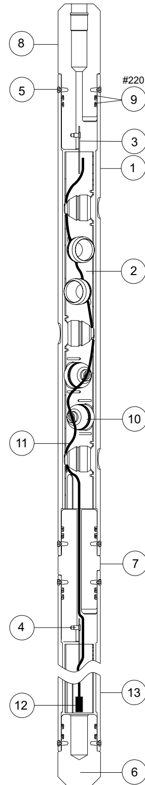
2-in. 4-spf 60° Slip-On Tube-Type
