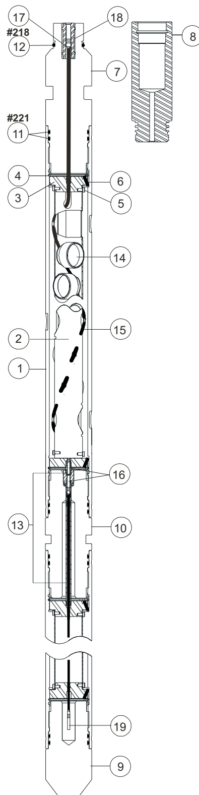
2-in. 6-spf 60° Scalloped System
