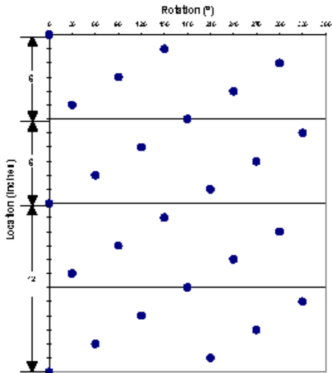
Shot Pattern for 4.625-in. 12-spf 30°/150° Phasing
