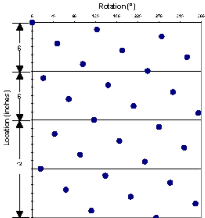
Shot Pattern for 6.5-in. 14-spf 138° Phasing
