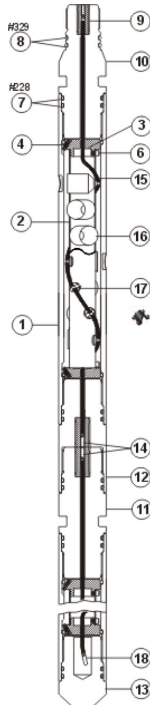
2 7/8-in. 6-spf 60° Millennium™ VannGun™ System
