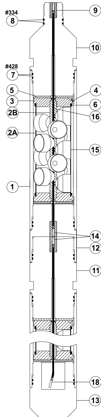
6-in. 12-spf 51.4°/154.2° VannGun™ System
