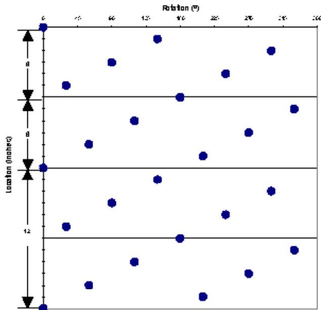
Shot Pattern for 4.75-in. 12-spf 30°/150° Phasing
