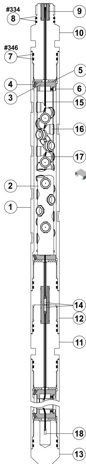
5-in. 12-spf 25.7°/128.5° SH VannGun™ System
