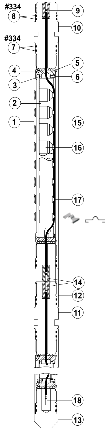
3 3/8-in. 5-spf 0° SDP VannGun™ System
