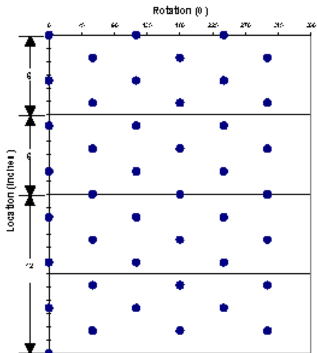
Shot Pattern for 5.125-in. 21-spf 60°/120° Phasing
