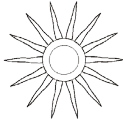
138° Phasing 14 Perforation Planes
