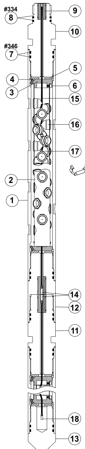
5 1/8-in. 12-spf OMNI™ VannGun™ System
