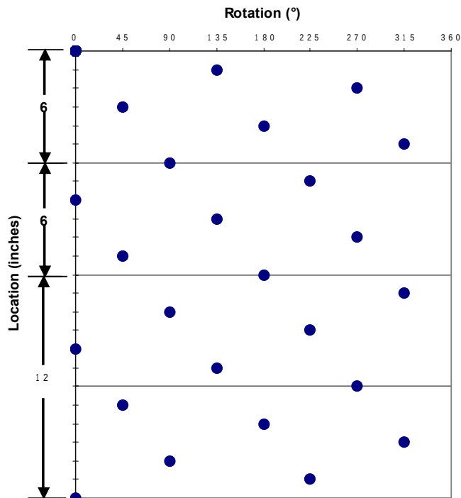
Shot Pattern for 7-in 12-spf 45°/135° Phasing
