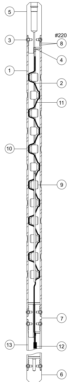
2-in. 6-spf 180° Slip-On Strip-Type
