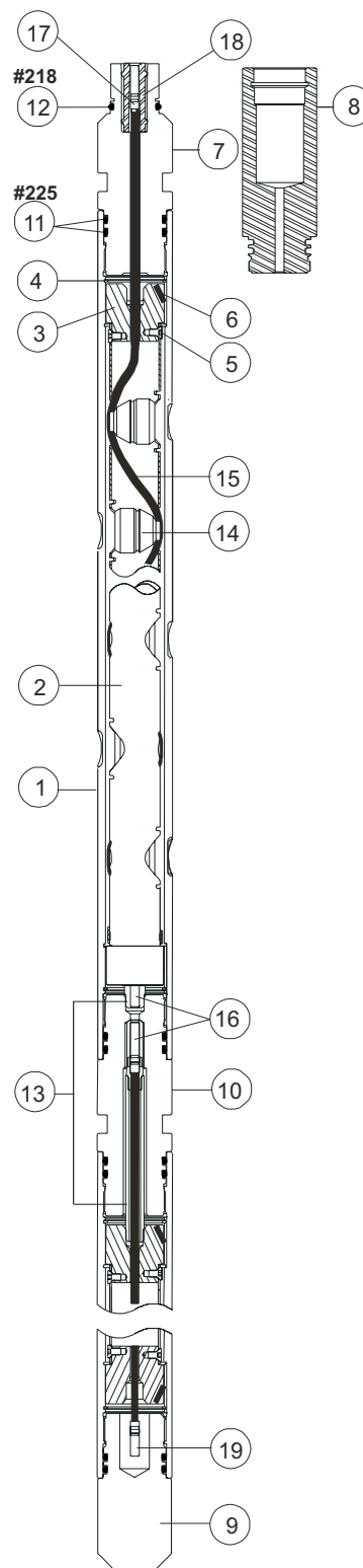
2 1/2-in. 4-spf 180° Scalloped System
