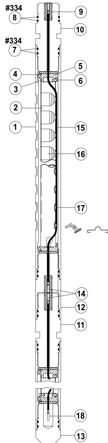
3 3/8-in. 5-spf 0° VannGun™ System
