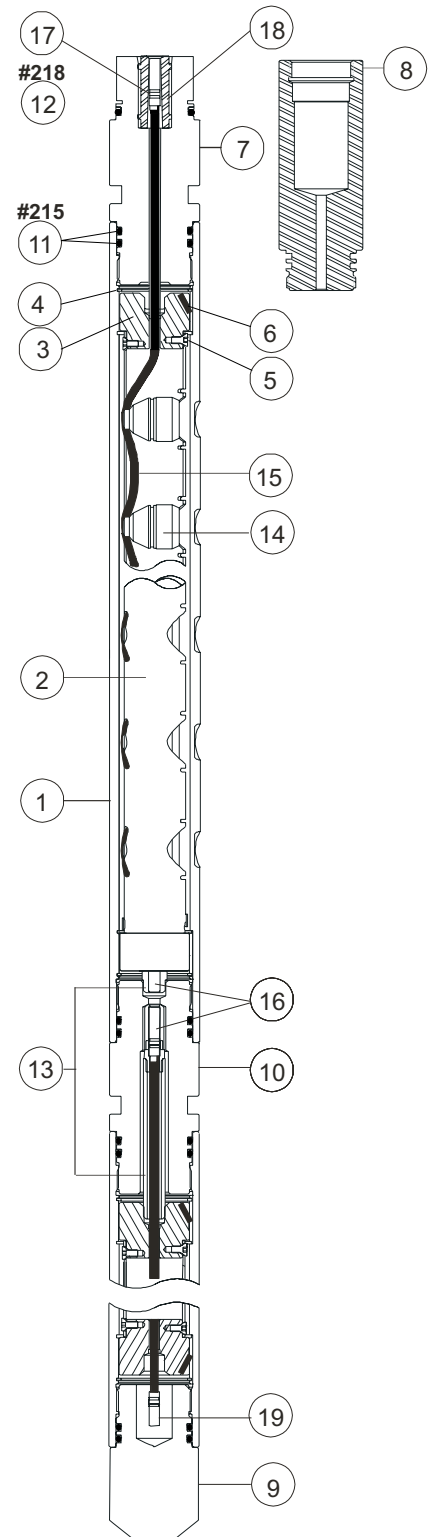
1 9/16-in. 6-spf 0° Scalloped System
