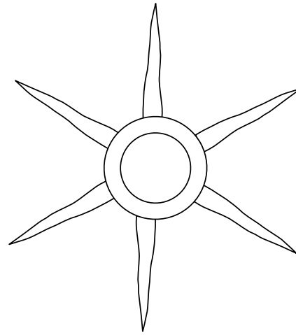
60° Phasing 6 Perforation Planes
