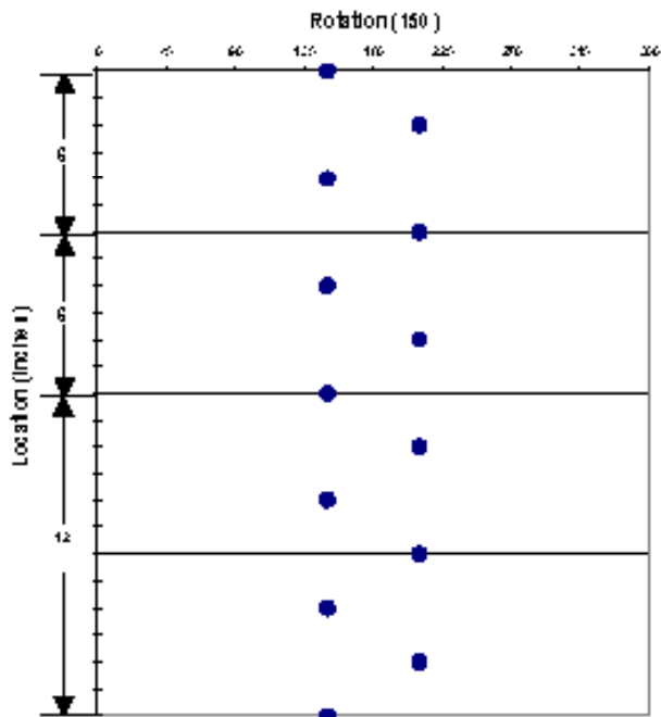
Shot Pattern for 3.375-in. 6-spf 60° Phasing
