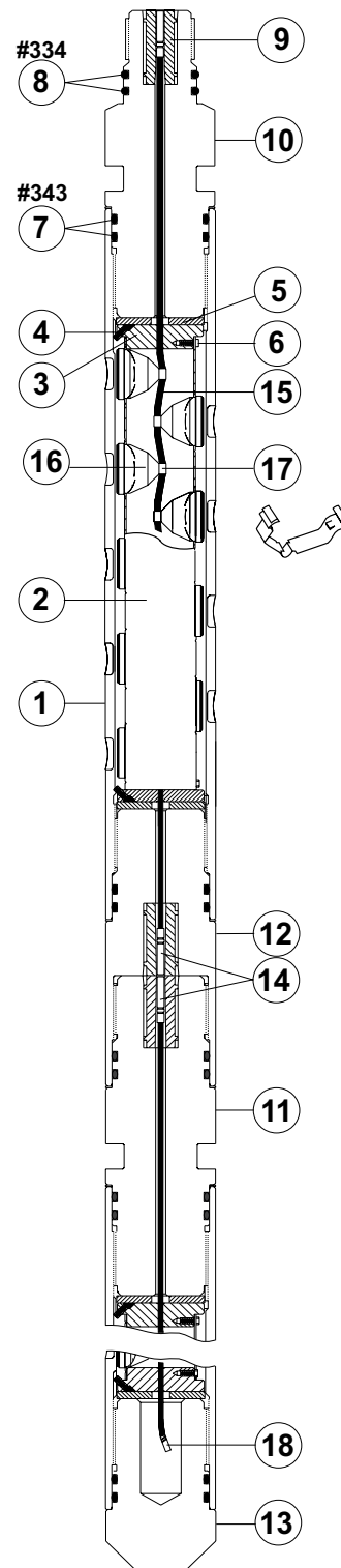
4 5/8-in. 8-spf 180° VannGun™ System
