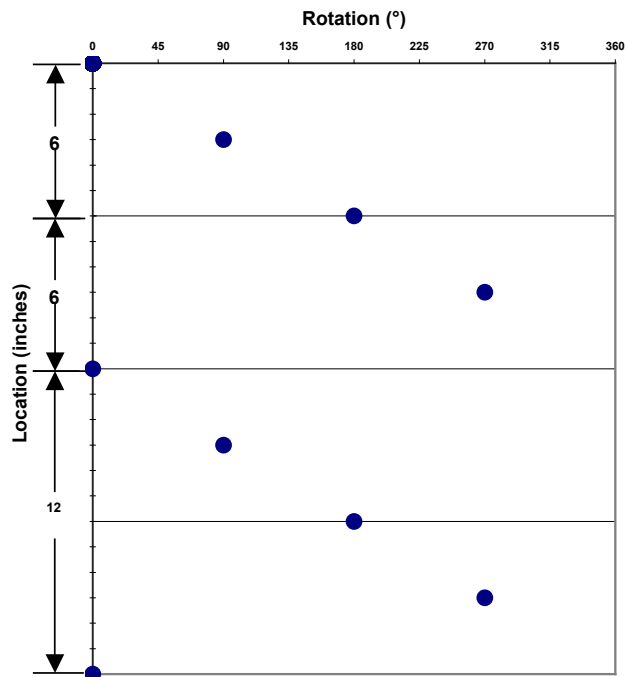
Shot Pattern for 3.375-in. 4-spf 90° Phasing
