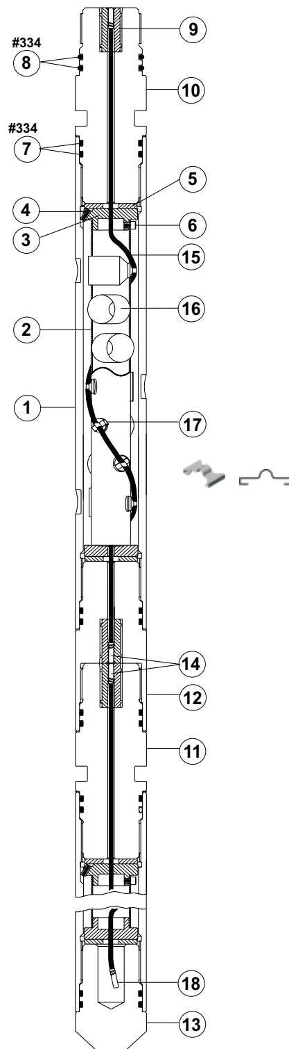
3 3/8-in. 6-spf 60° VannGun™ System
