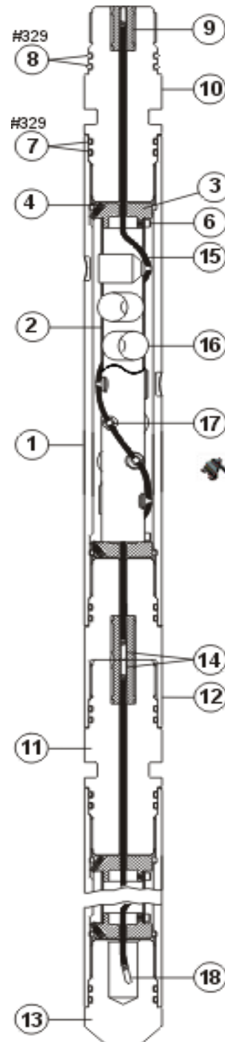
2 3/4-in. 6-spf 60° Millennium™ VannGun™ System
