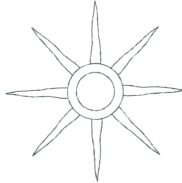
45°/135° Phasing 8 Perforation Planes
