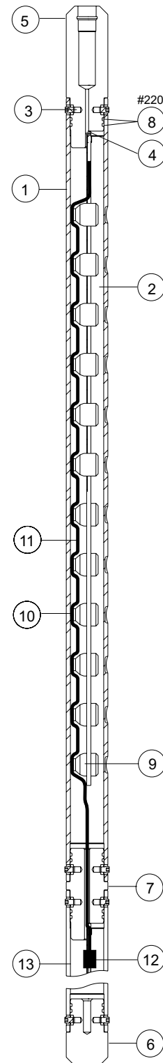
2-in. 4-spf 0° Slip-On Tubing Puncher
