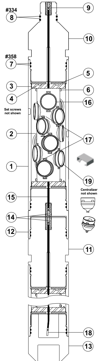
6 1/2-in. 14-spf 138° VannGun™ System
