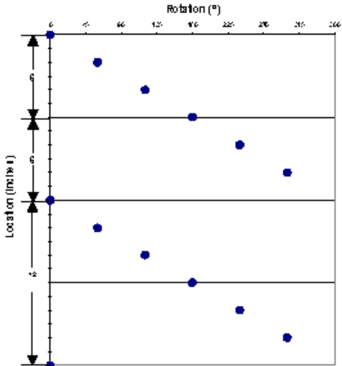
Shot Pattern for 4.625-in. 6-spf 60° Phasing
