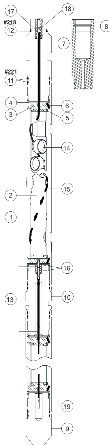
2-in. 4-spf 60° Scalloped System
