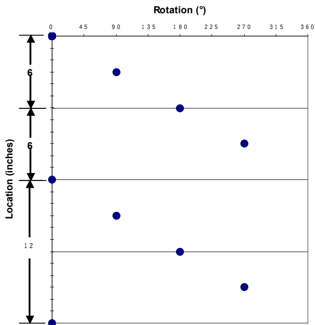
Shot Pattern for 4-in. 4-spf 90° Phasing
