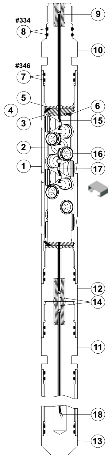
5-in. 12-spf 45°/135° MIRAGE™ SH VannGun® System
