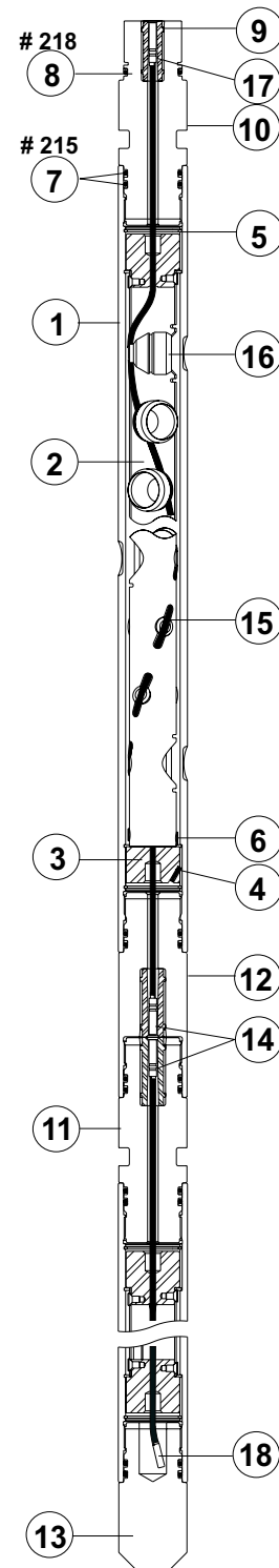
1 9/16-in. 6-spf 60° VannGun™ System
