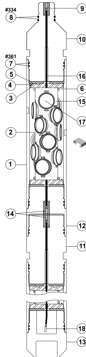
7-in. 12-spf 45°/135° MaxForce™ VannGun™ System
