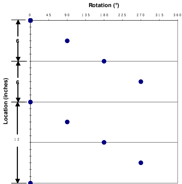
Shot Pattern for 4-in. 4-spf 90° Phasing
