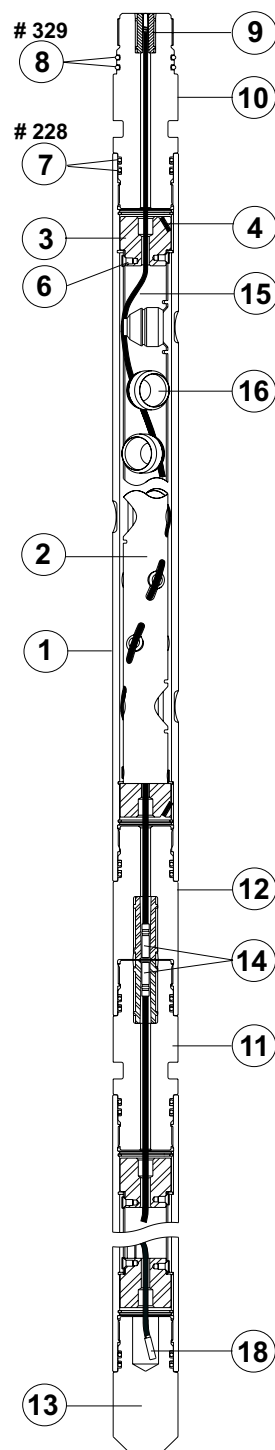
2 7/8-in. 4-spf 60° VannGun™ System
