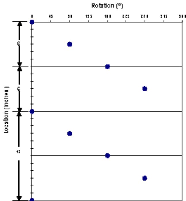
Shot Pattern for 2-in. 4-spf 90° Phasing
