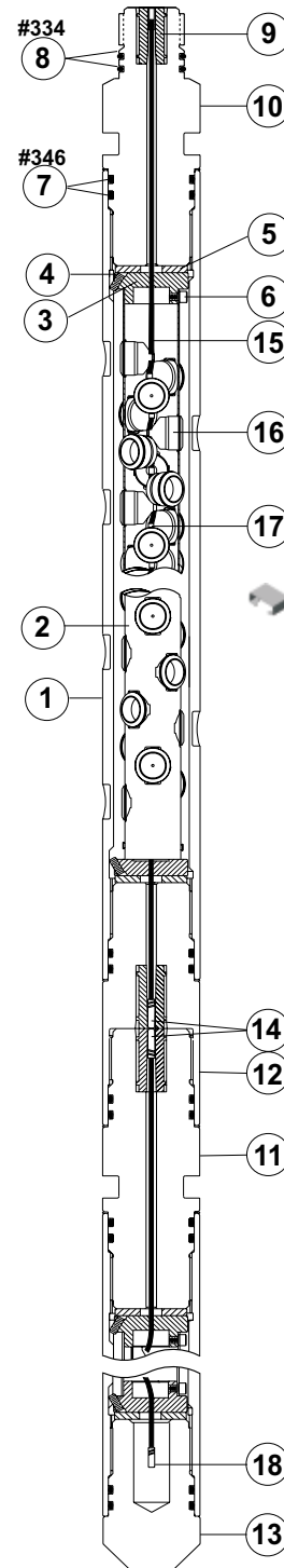
5 1/8 in. 14-spf 25.7°/128.5° SH VannGun™ System
