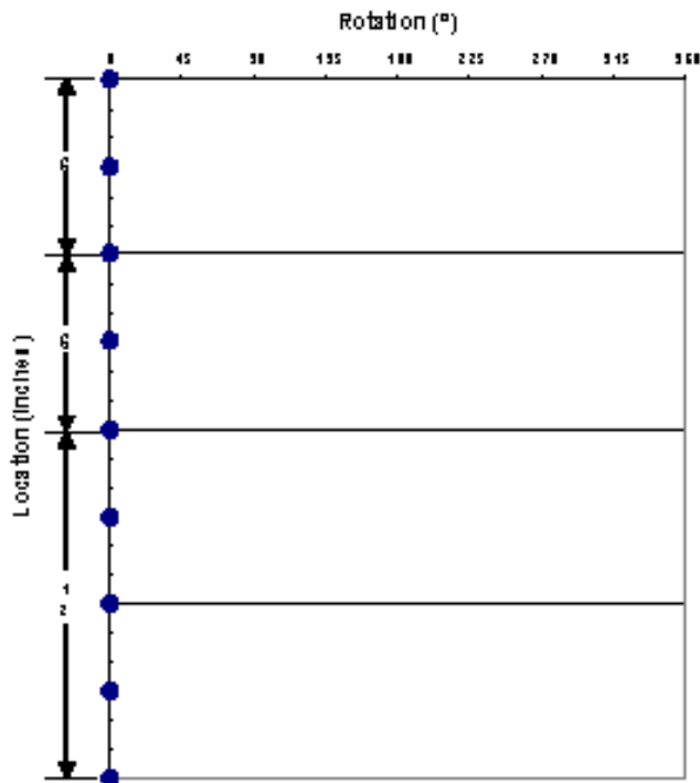
Shot Pattern for 1.5625-in. 4-spf 0° Phasing
