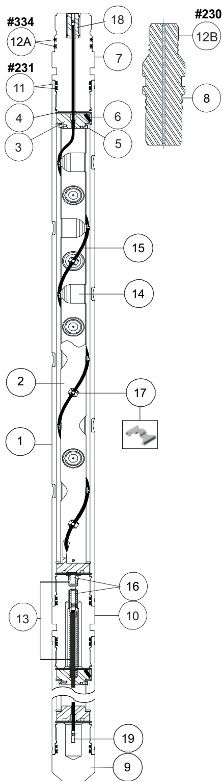
3 3/8-in. 4-spf 90° Scalloped System
