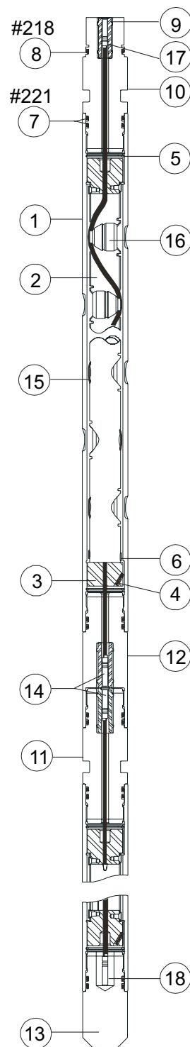
2-in. 4-spf 180° VannGun™ System
