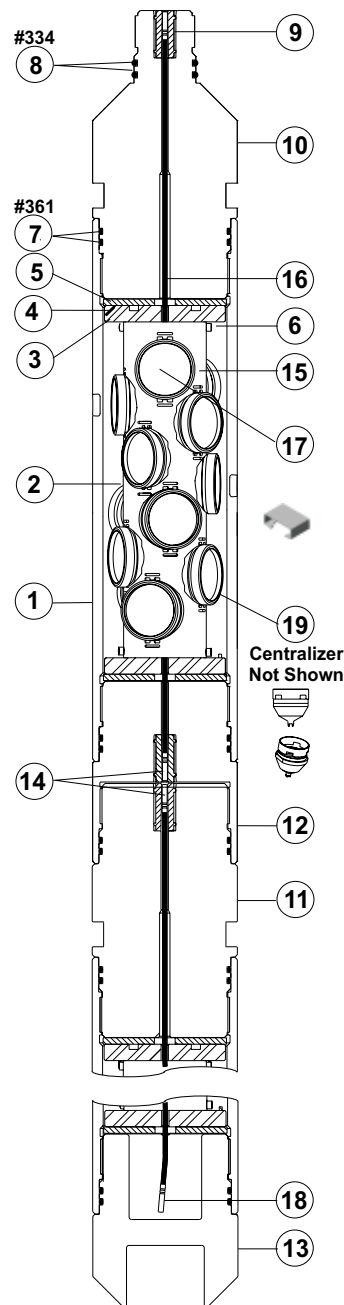
7-in. 12-spf 45°/135° DP VannGun™ System
