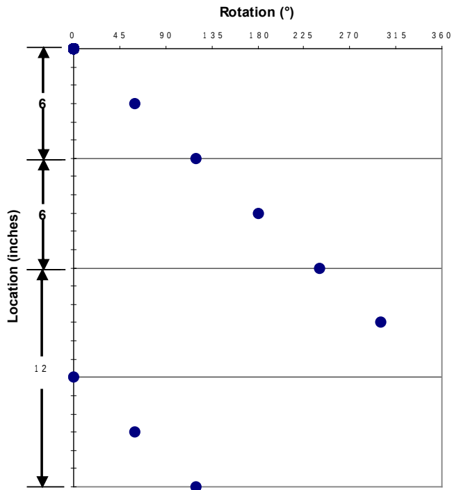
Shot Pattern for 2.375-in. 4-spf 60° Phasing
