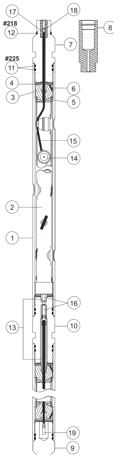
2 1/2-in. 4-spf 90° Scalloped System
