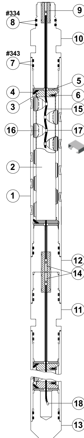
4 5/8-in. 8-spf 180° SH VannGun™ System
