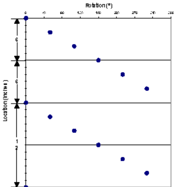
60° Phasing 6 Perforation Planes
