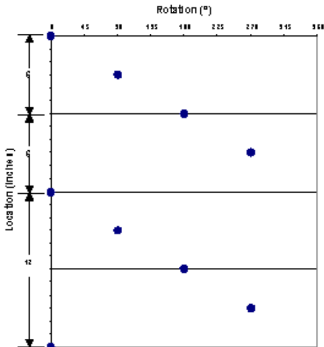
Shot Pattern for 2.5-in. 4-spf 90° Phasing
