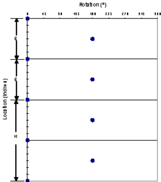
Shot Pattern for 1.5625-in. 4-spf 180° Phasing
