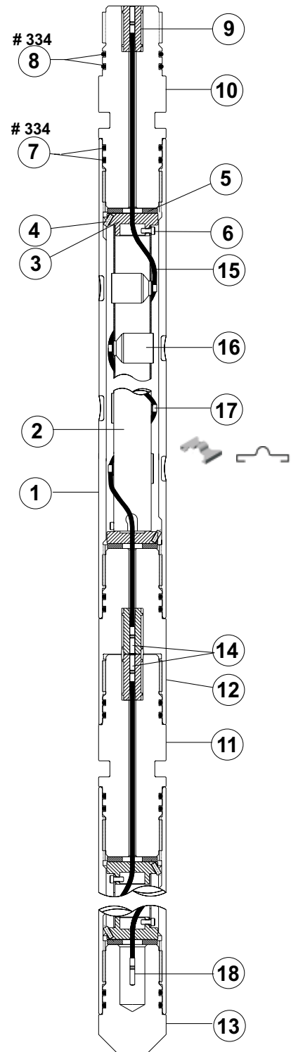
3 3/8-in. 4-spf 180° SDP VannGun™ System
