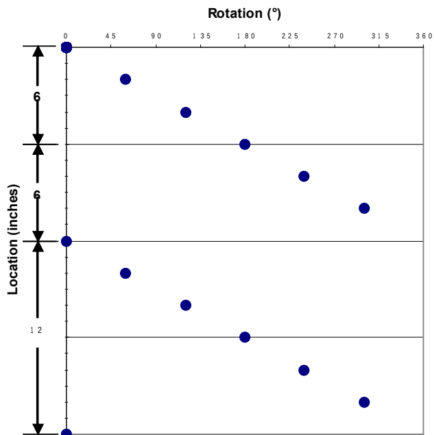
Shot Pattern for 3.375-in. 6-spf 60° Phasing
