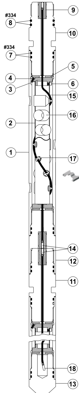
3 3/8-in. 6-spf 60° SDP VannGun™ System
