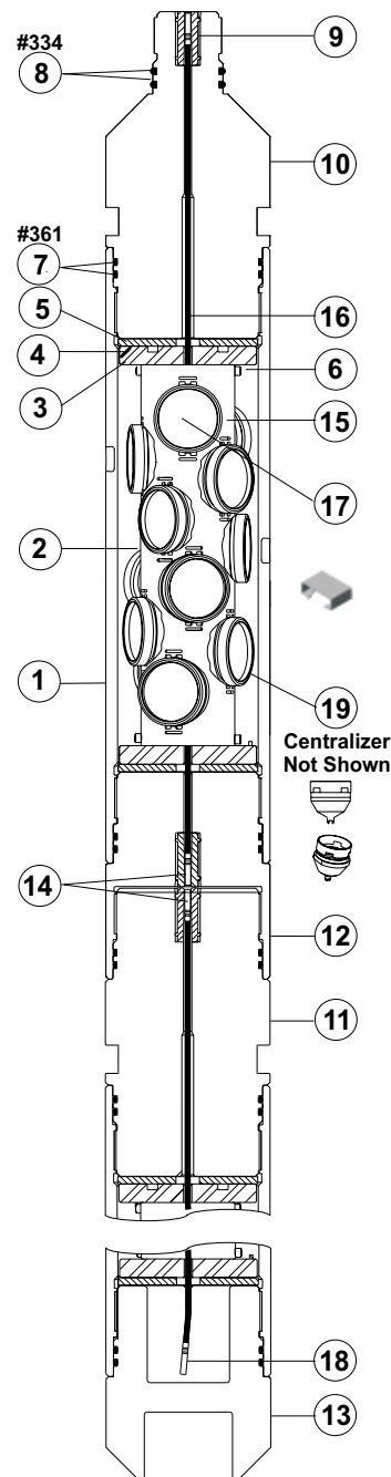
7-in. 14-spf 138° BH/SH VannGun™ System
