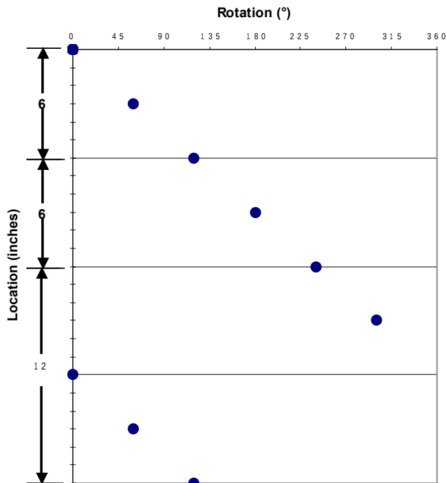
Shot Pattern for 2-in. 4-spf 60° Phasing
