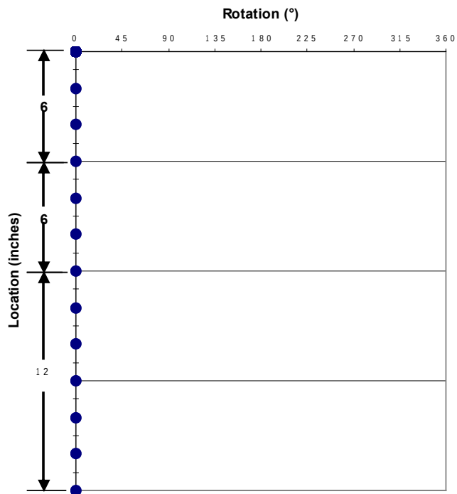
Shot Pattern for 1.5625-in. 6-spf 0° Phasing
