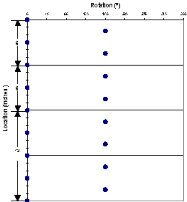
Shot Pattern for 3.375-in. 8-spf 180° Phasing
