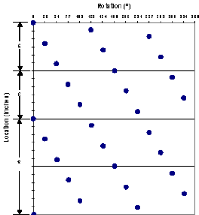
Shot Pattern for 5-in. 14-spf 25.7°/128.5° Phasing
