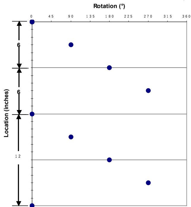
Shot Pattern for 1.5625-in. 4-spf 90° Phasing
