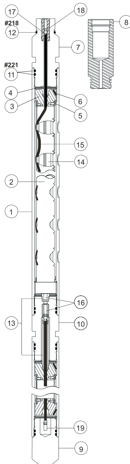
2-in. 6-spf 0° Scalloped System
