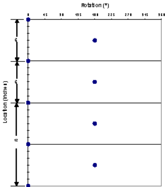
Shot Pattern for 2-in. 4-spf 180° Phasing
