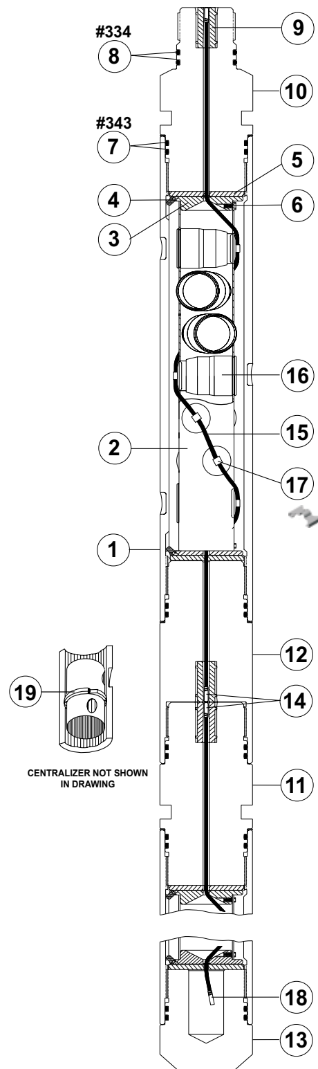
4 5/8-in. 6-spf 60° (12-spf Carrier) VannGun™ System
