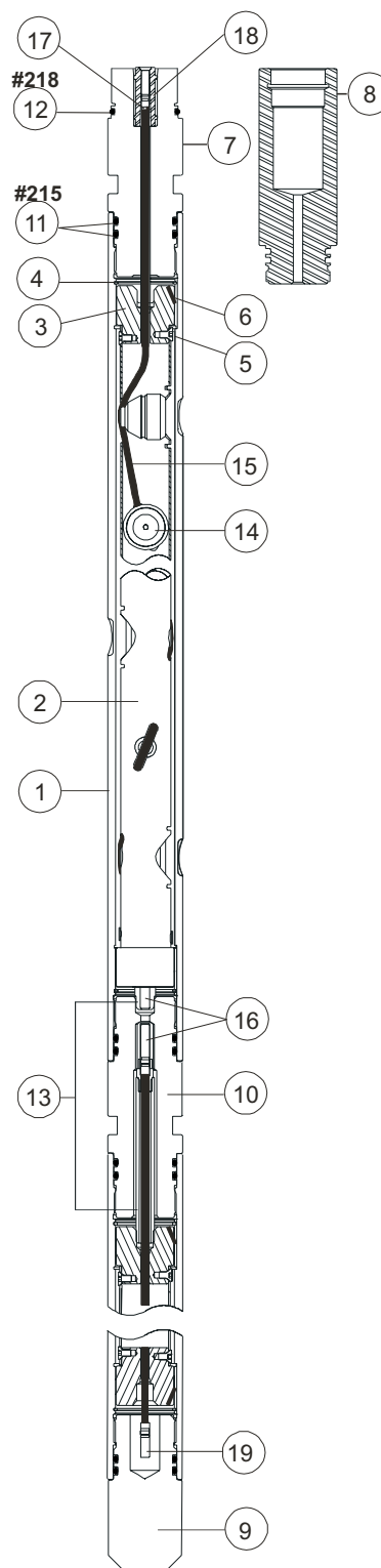
1 9/16-in. 4-spf 90° Scalloped System
