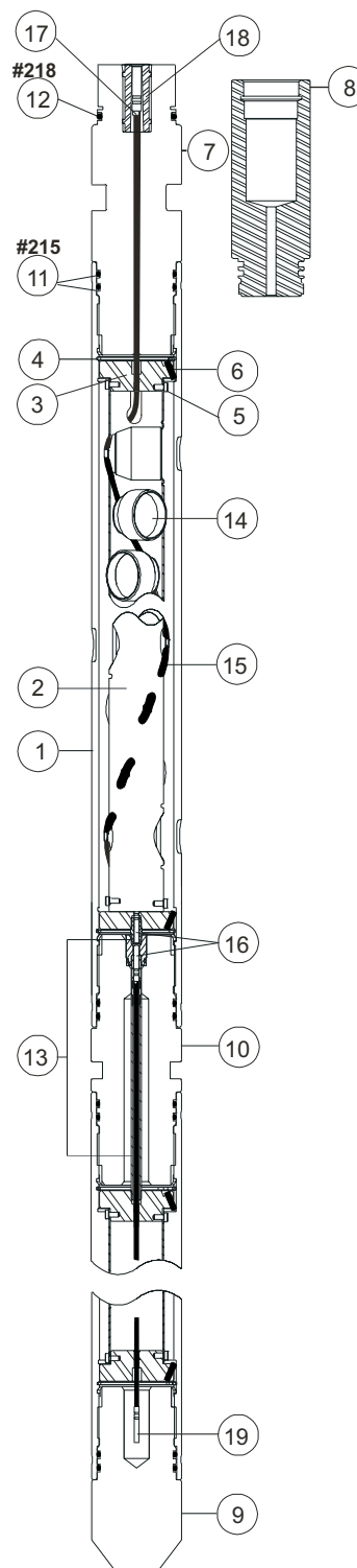
1 9/16-in. 4-spf 60° Scalloped System
