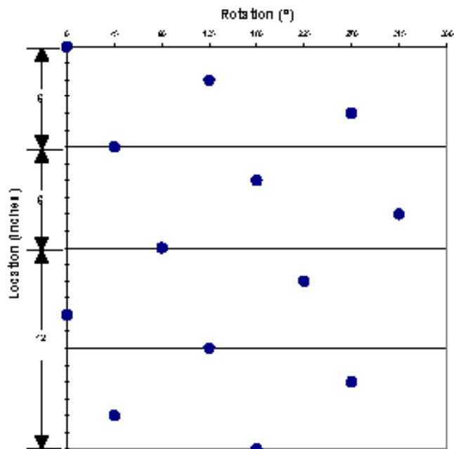
Shot Pattern for 5.125-in. 6-spf 135° Phasing
