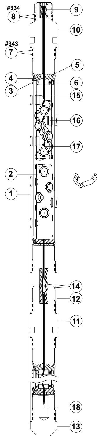
4 5/8-in. 12-spf OMNI™ VannGun™ System
