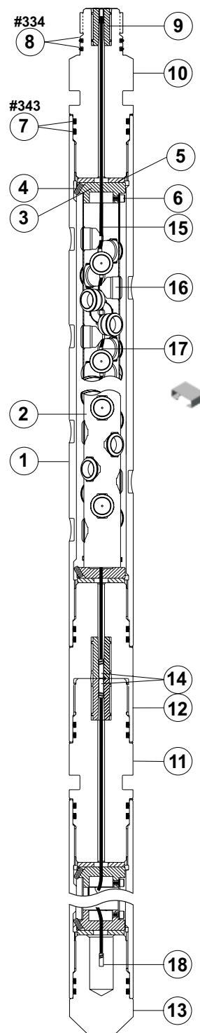
4 5/8-in. 14-spf 25.7°/128.5° SH VannGun™ System
