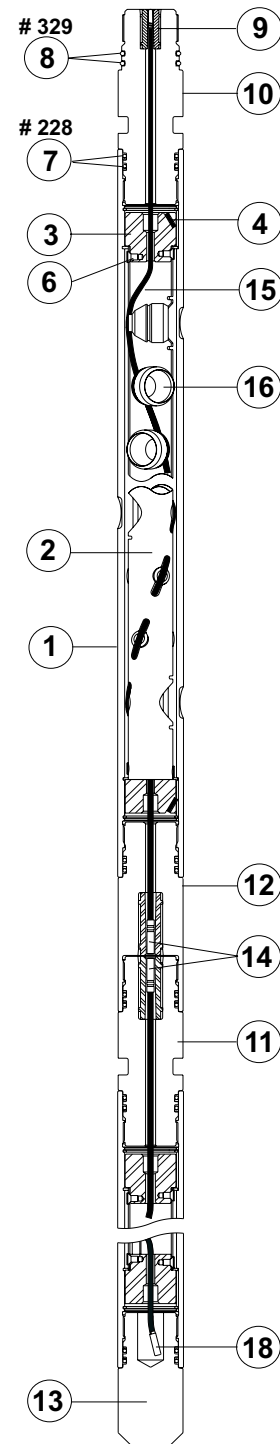
2 7/8-in. 6-spf 60° Millennium VannGun™ System
