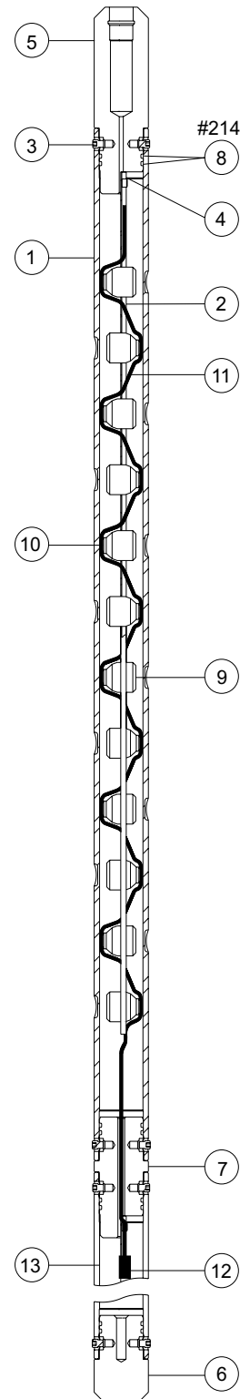
1 9/16-in. 4-spf 180° Slip-On Strip-Type
