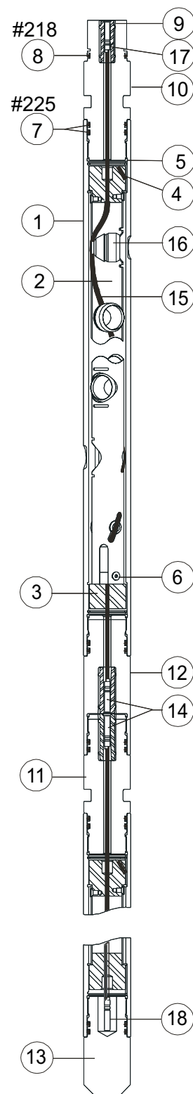
2 1/2-in. 4-spf 60° VannGun™ System
