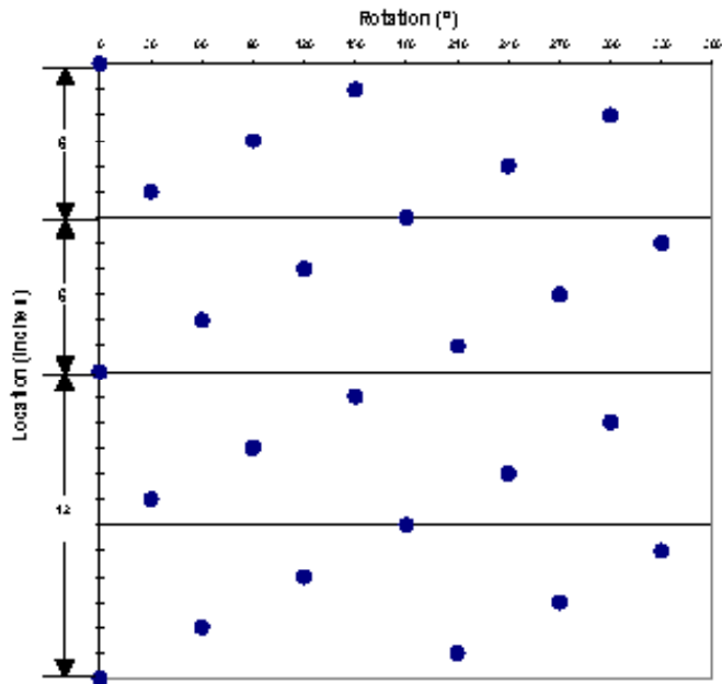
Shot Pattern for 5.125-in. 12-spf 30°/150° Phasing
