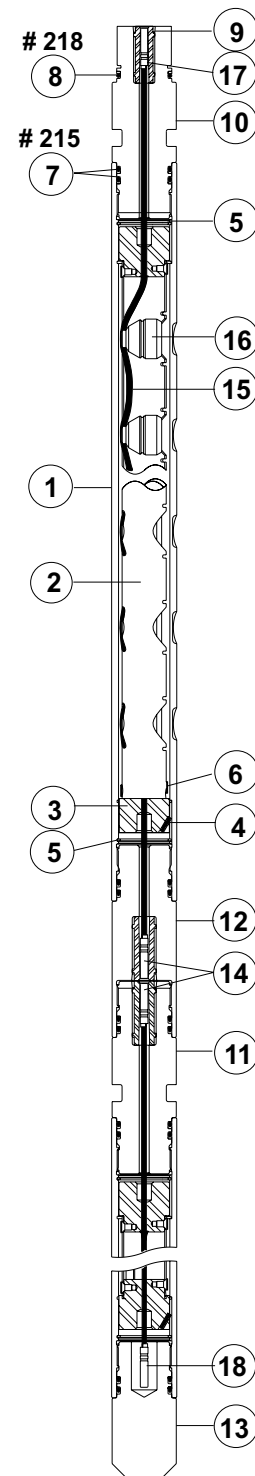
1 9/16-in. 4-spf 0° VannGun™ System
