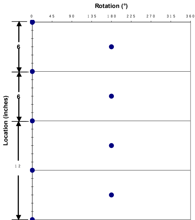
Shot Pattern for 2.5-in. 4-spf 180° Phasing
