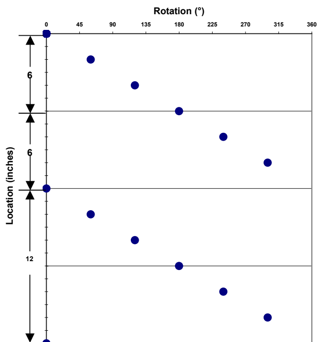
Shot Pattern for 2.875-in. 6-spf 60° Phasing
