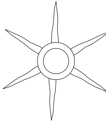
60°/120° Phasing 6 Perforation Planes
