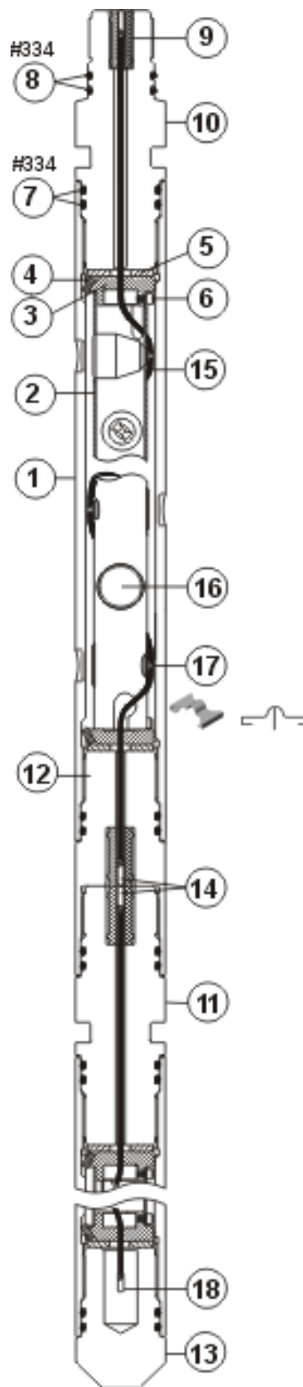
3 3/8-in. 4-spf 90° SDP VannGun™ System
