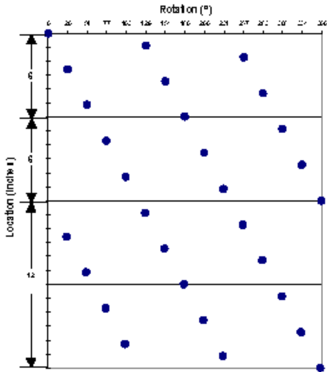
Shot Pattern for 4.625-in. 14-spf 25.7°/128.5° Phasing
