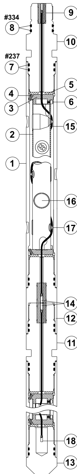
4-in. 4-spf 90° VannGun™ System
