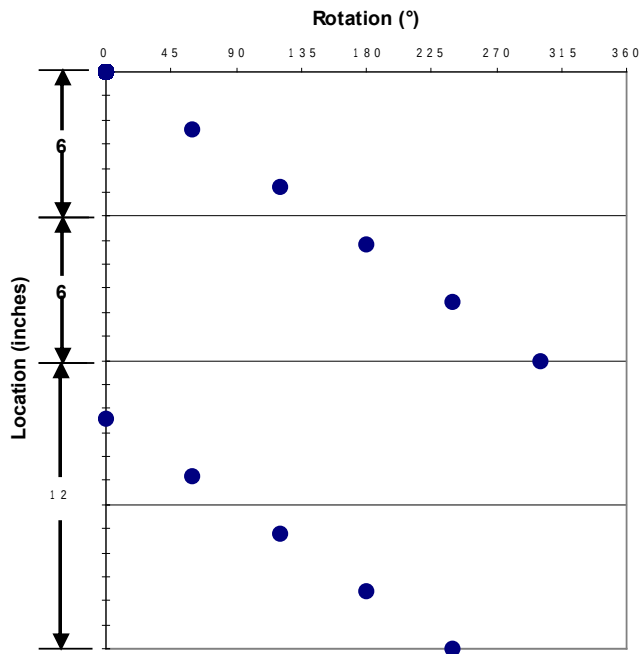
Shot Pattern for 4-in. 4-spf 60° Phasing
