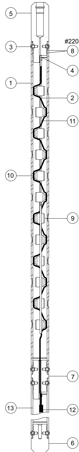
2-in. 4-spf 180° Slip-On Strip-Type
