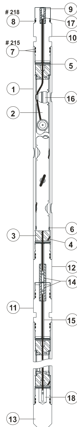
1 9/16-in. 4-spf 90° VannGun™ System
