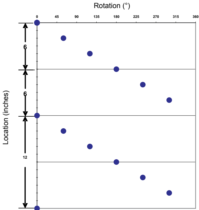
Shot Pattern for 2.875-in. 4-spf 60° Phasing
