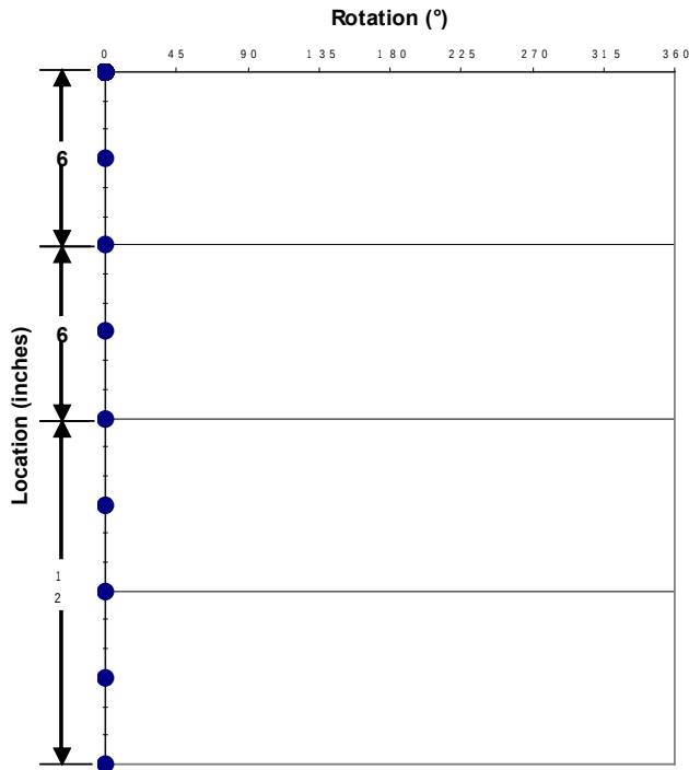
Shot Patterns for 1.5625-in. 4-spf 0° Phasing
