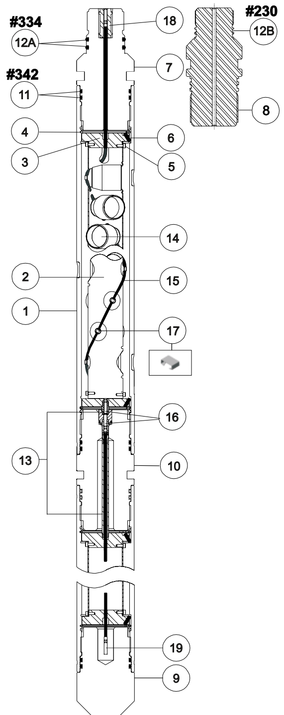
4 1/2-in. 5-spf 60° Scalloped System
