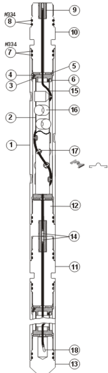
3 3/8-in. 4-spf 60° SDP VannGun™ System
