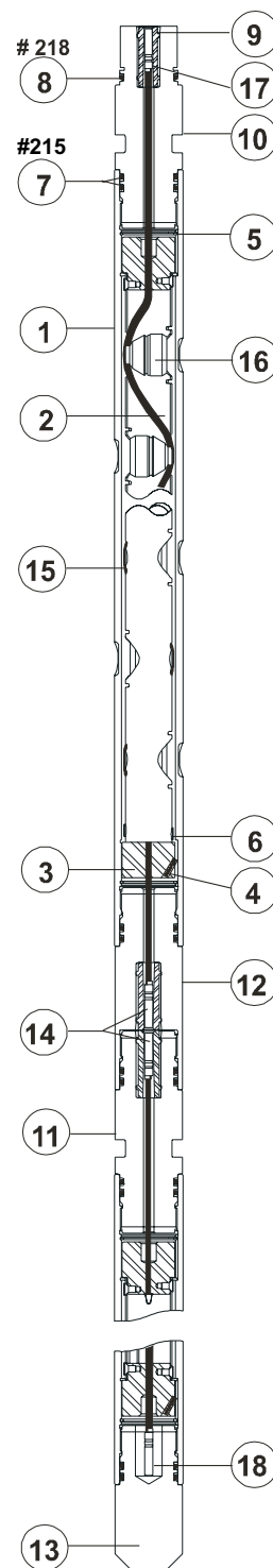
1 9/16-in. 4-spf 180° VannGun™ System
