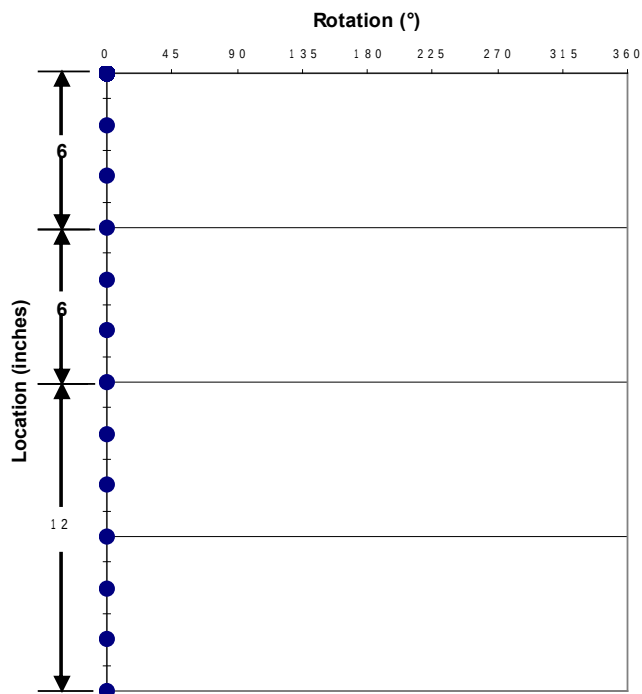
Shot Pattern for 2-in. 6-spf 0° Phasing
