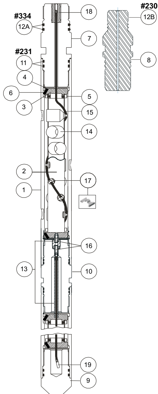
3 3/8-in. 6-spf 60° Scalloped System
