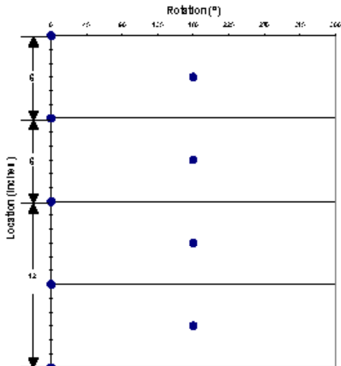
Shot Pattern for 4.625-in. 4-spf 180° Phasing
