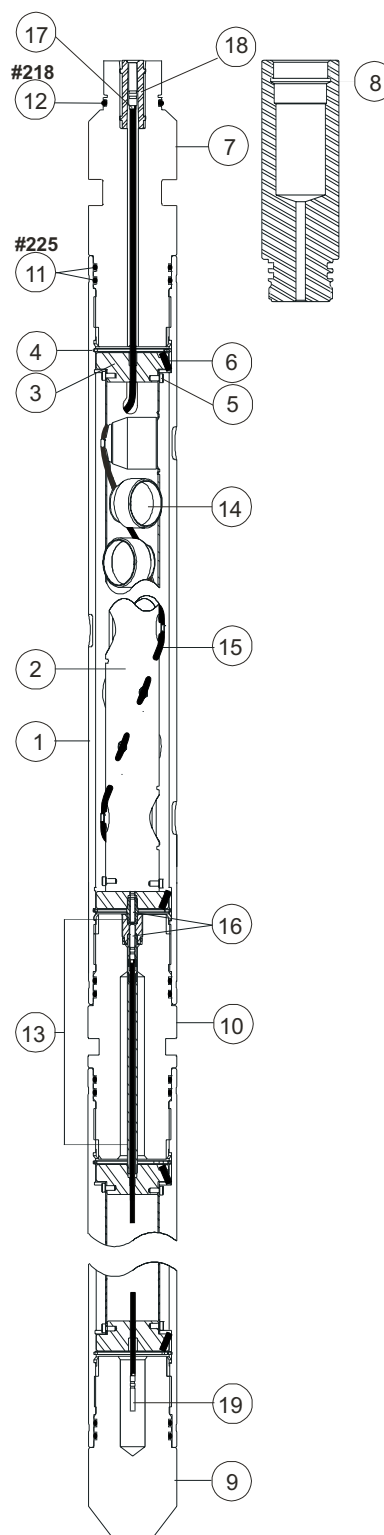
2 1/2-in. 4-spf 60° Scalloped System
