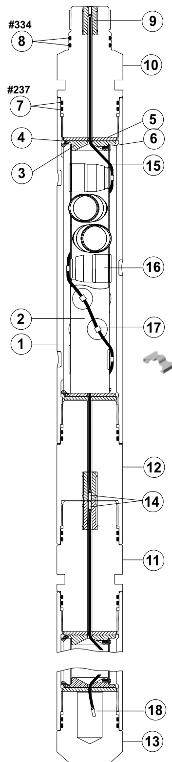
4-in. 6-spf 60° VannGun™ System
