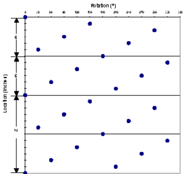
Shot Pattern for 5.125-in. 12-spf 30°/150° Phasing
