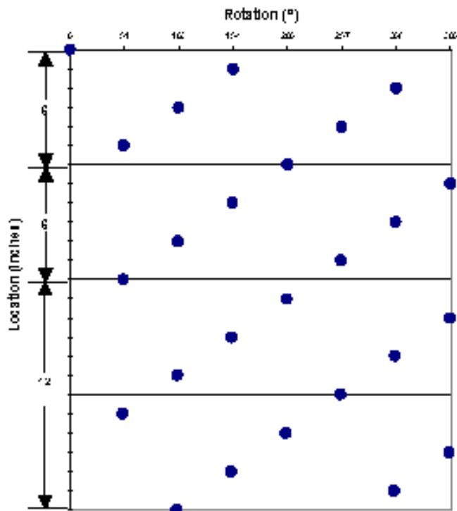
Shot Pattern for 6-in. 12-spf 51.4°/154.2° Phasing
