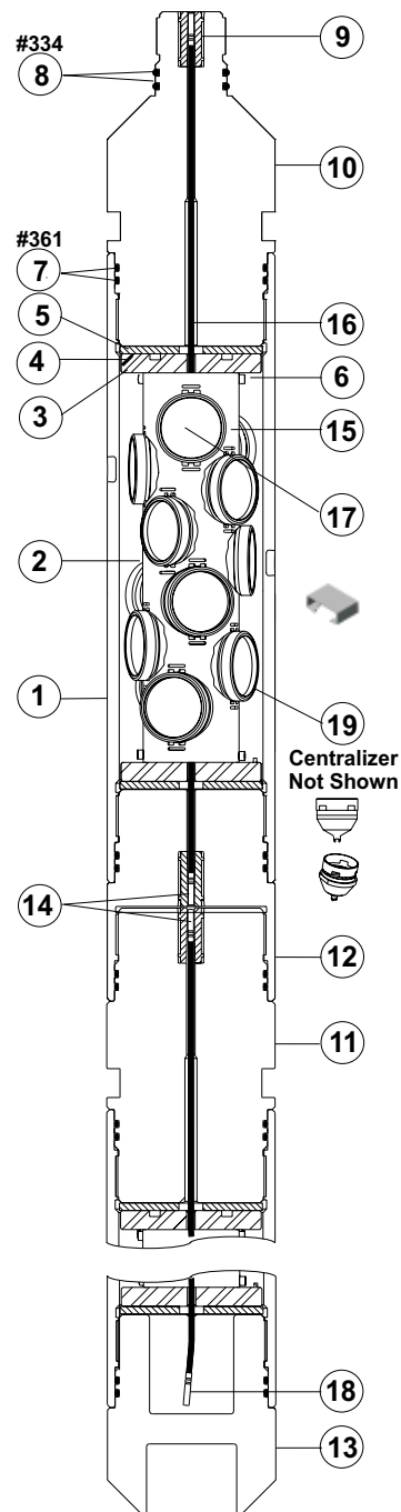
7-in. 12-spf 45°/135° BH/SH VannGun™ System
