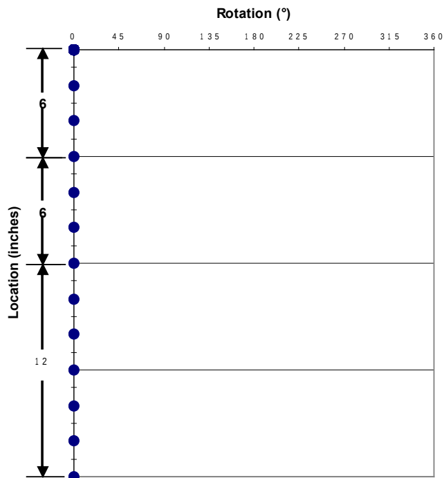
Shot Pattern for 2.5-in. 6-spf 0° Phasing
