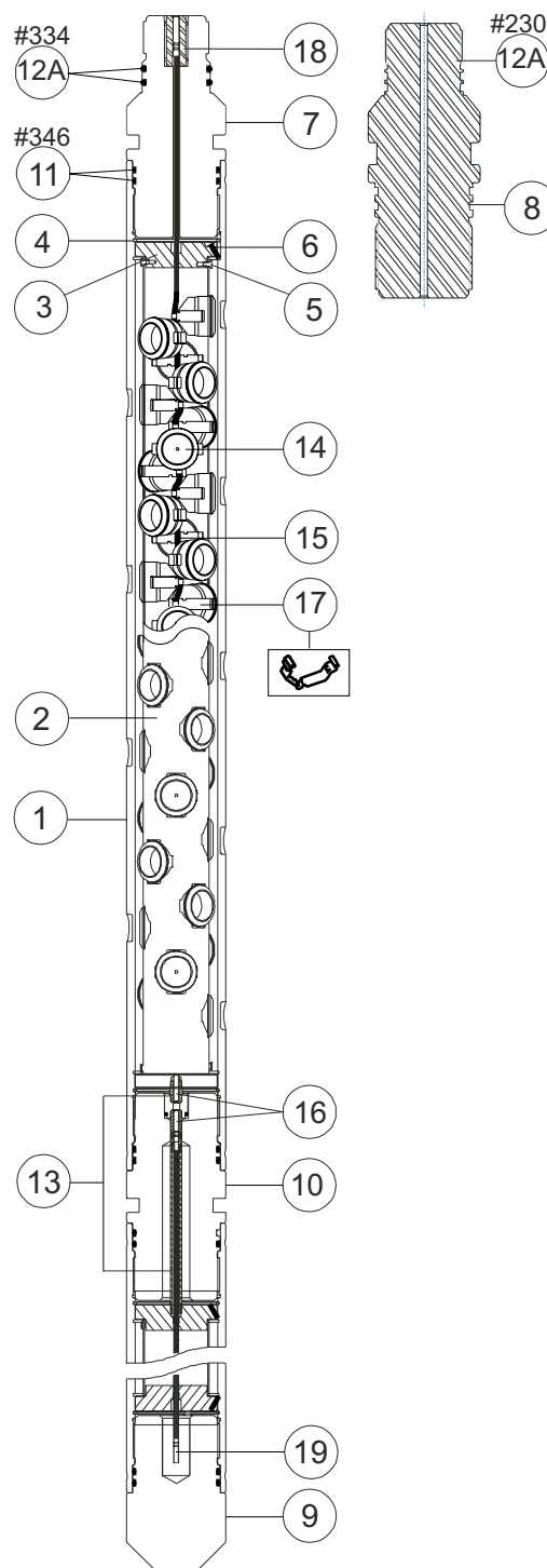
5 1/8-in. 12-spf 30°/150° Scalloped System
