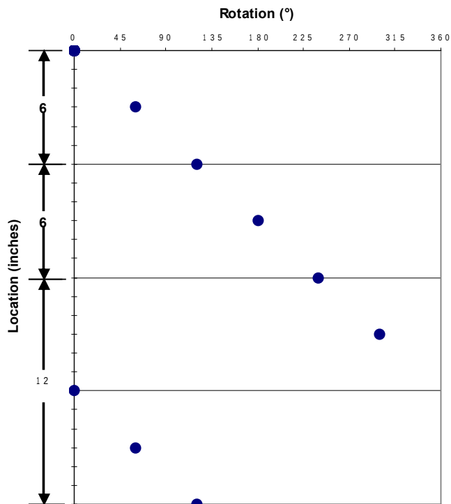
Shot Pattern for 1.5625-in. 4-spf 60° Phasing
