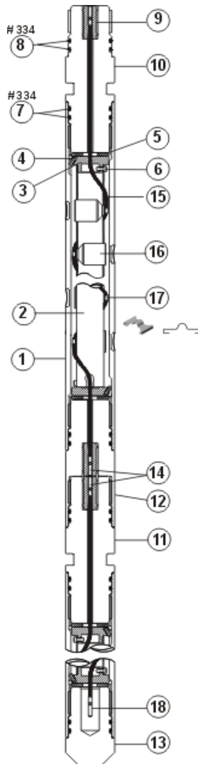
3 3/8-in. 4-spf 180° VannGun™ System
