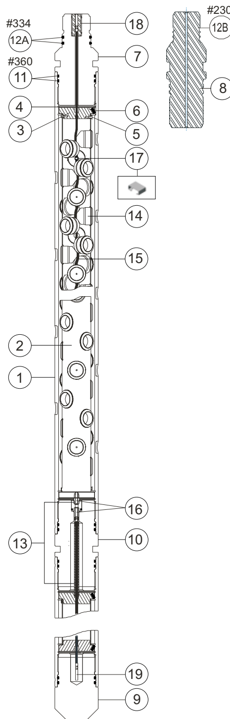
7-in. 12-spf 45°/135° Millennium™ System
