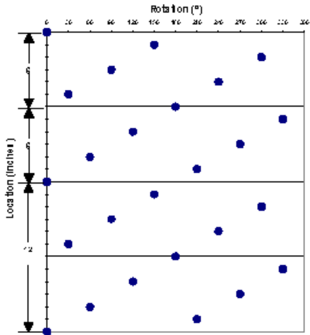
Shot Pattern for 5-in. 12-spf 30°/150° Phasing
