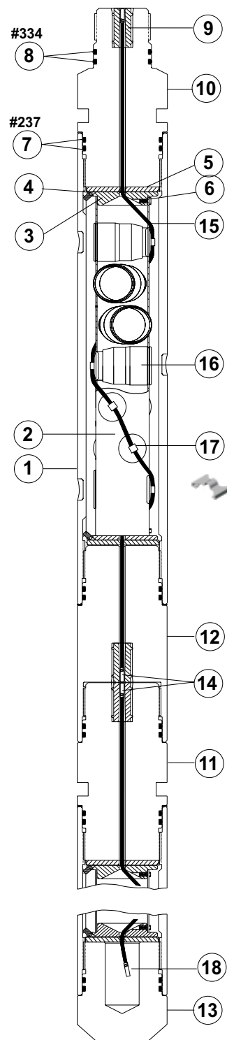
4-in. 4-spf 60° VannGun™ System
