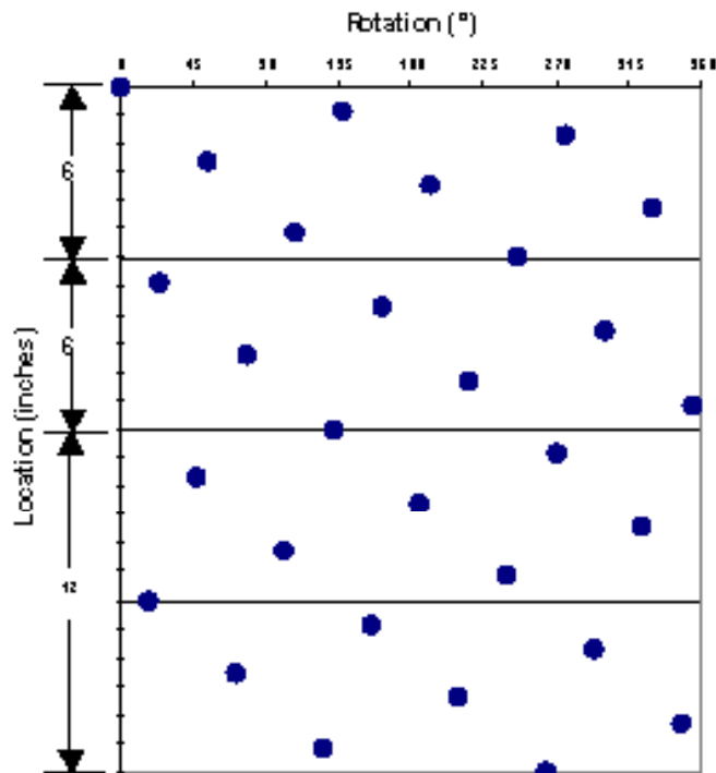
Shot Pattern for 7-in. 14-spf 138° Phasing
