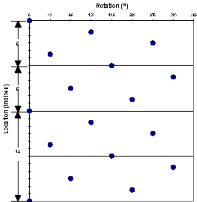
Shot Pattern for 4.625-in. 8-spf 45°/135° Phasing
