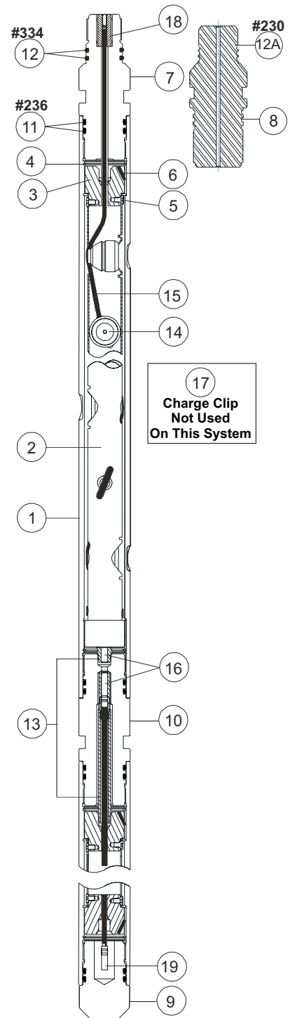
4-in. 4-spf 90° Scalloped System
