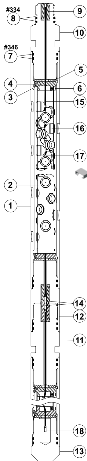
5 -in. 12-spf OMNI™ SH VannGun™ System
