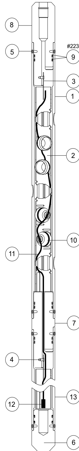
2 3/8-in. 6-spf 60° Slip-On Tube-Type
