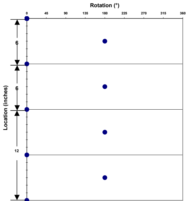
Shot Pattern for 2.75-in. 4-spf 180° Phasing
