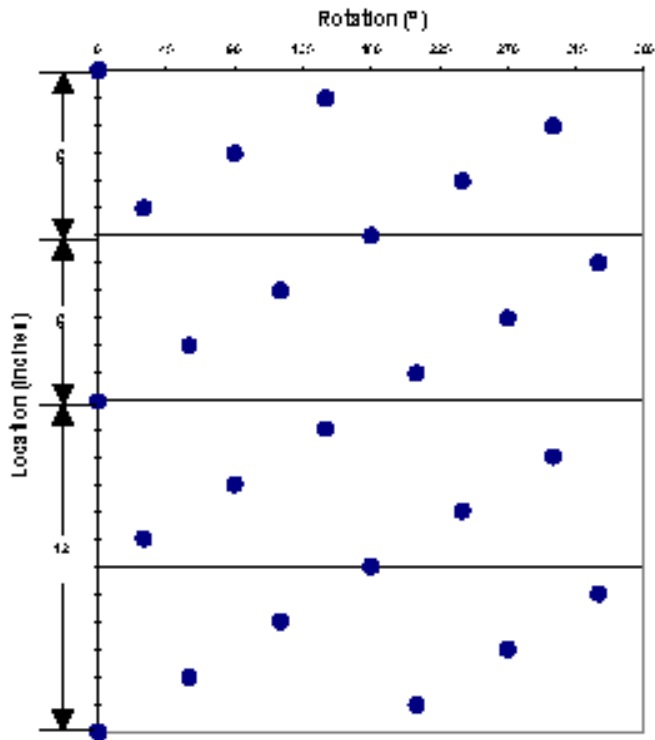
Shot Pattern for 3.375-in. 12-spf 30/150 Phasing
