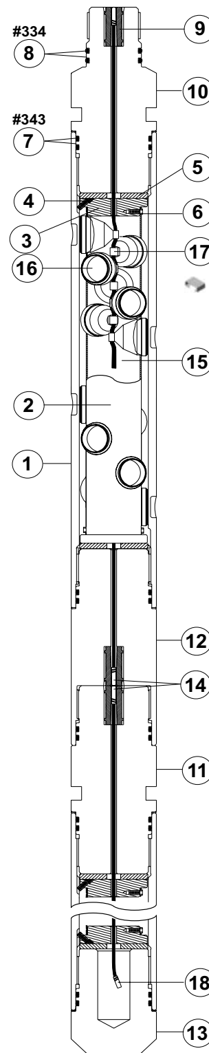
4 5/8-in. 8-spf 45°/135° SH VannGun™ System
