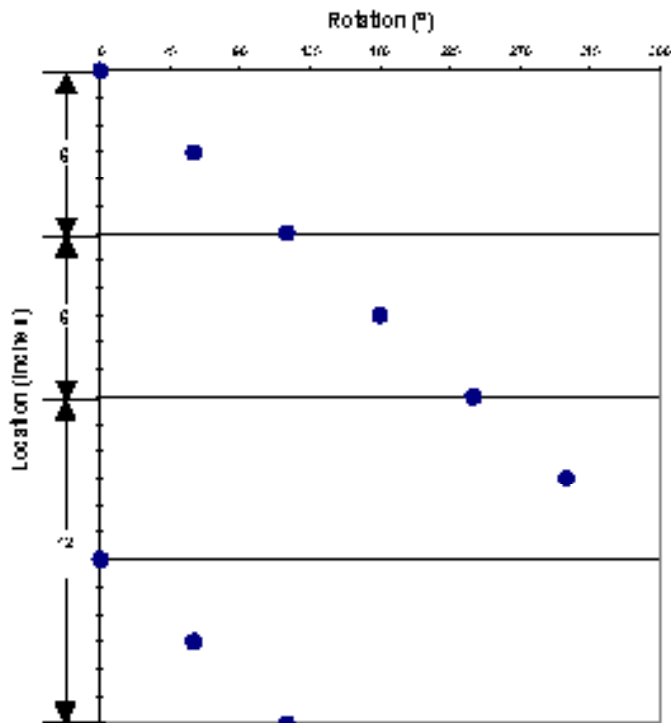
Shot Pattern for 4-in. 4-spf 60° Phasing
