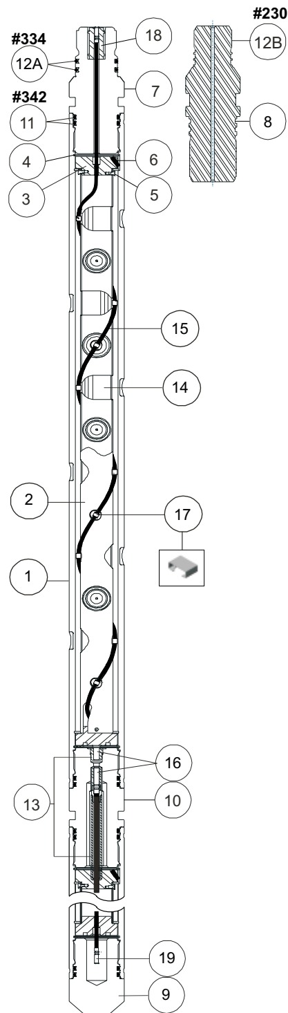
4 1/2-in. 4-spf 90° Scalloped System
