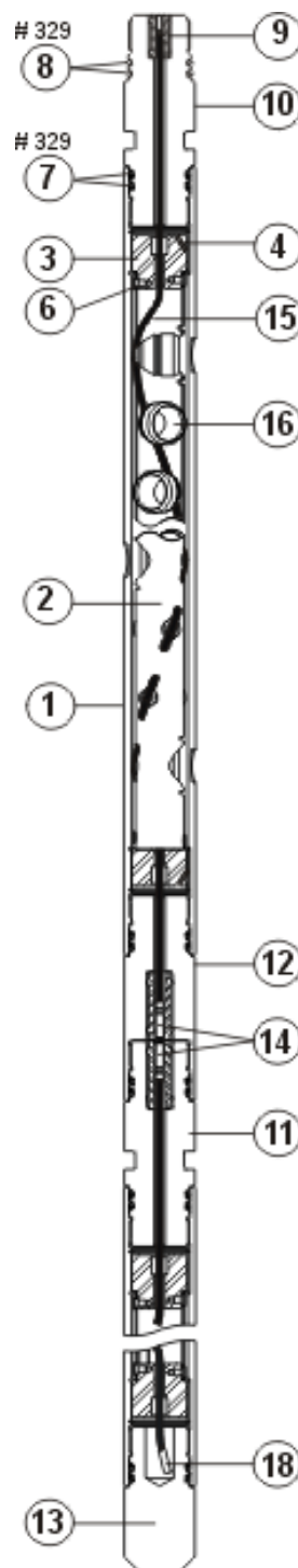
2 3/4-in. 6-spf 60° SDP VannGun™ System
