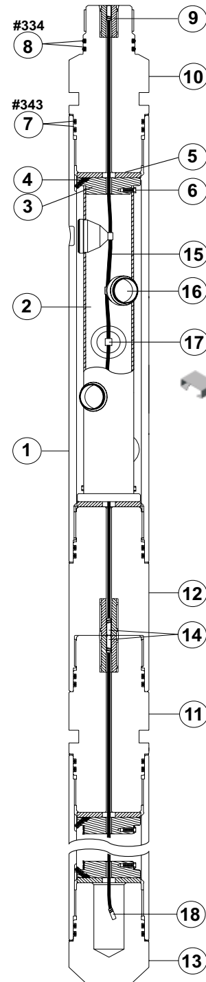
4 5/8-in. 5-spf 135° SH VannGun™ System
