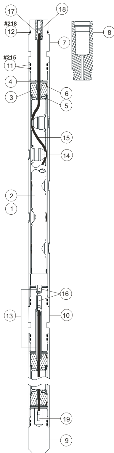
1 9/16-in. 4-spf 180° Scalloped System
