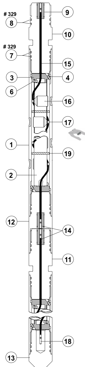
2 3/4-in. 5-spf 180° VannGun™ System
