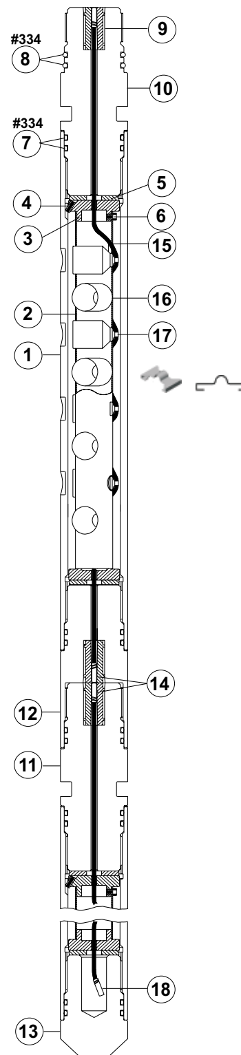
3 3/8-in. 6-spf 60° Lowside VannGun™ System
