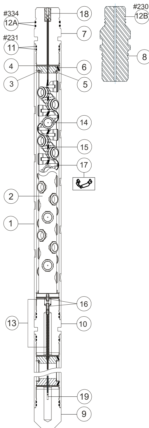
3 3/8-in. 12-spf Omni™ System
