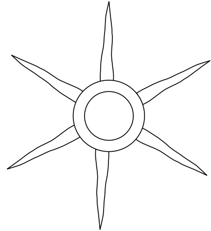
60° Phasing 6 Perforation Planes
