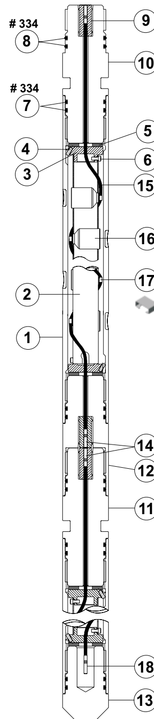
3 3/8-in. 8-spf 180° VannGun™ System
