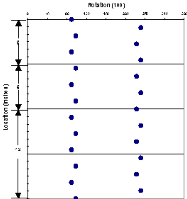
Shot Pattern for 4.625-in. 11-spf 140°/160° Phasing
