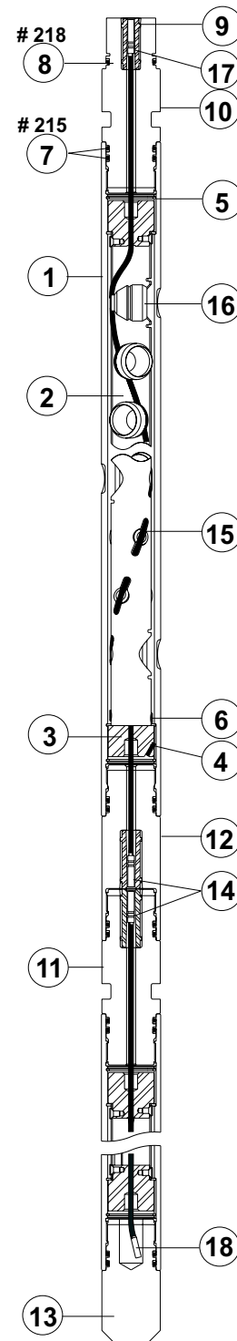
1 9/16-in. 4-spf 60° VannGun™ System
