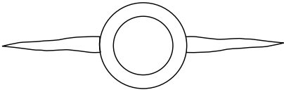
180° Phasing 2 Perforation Planes
