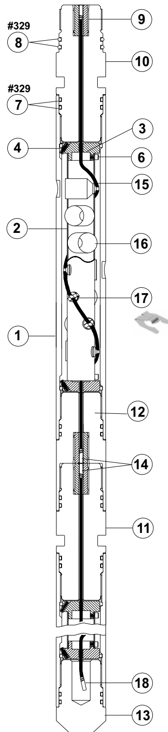
2 3/4-in. 6-spf 60° VannGun™ System
