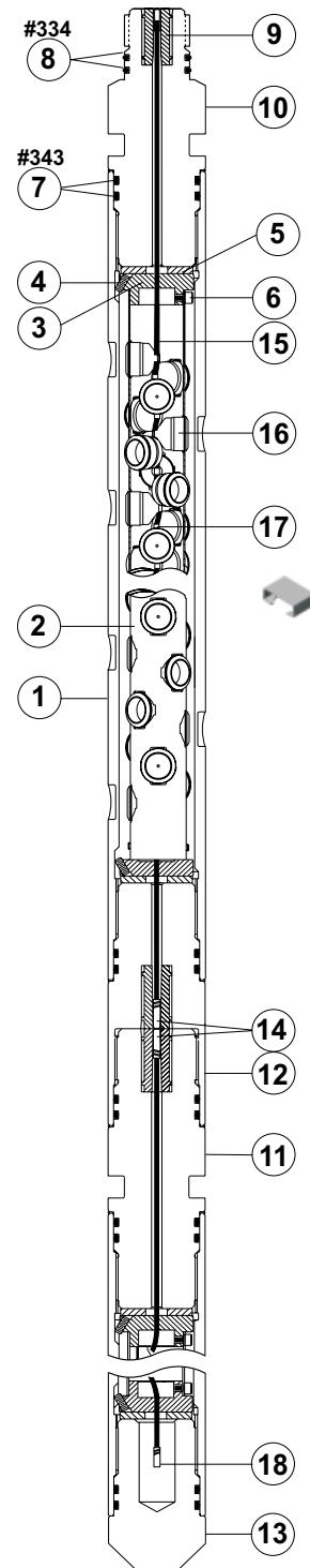
4 5/8-in. 18-spf 45°/135° DP VannGun™ System
