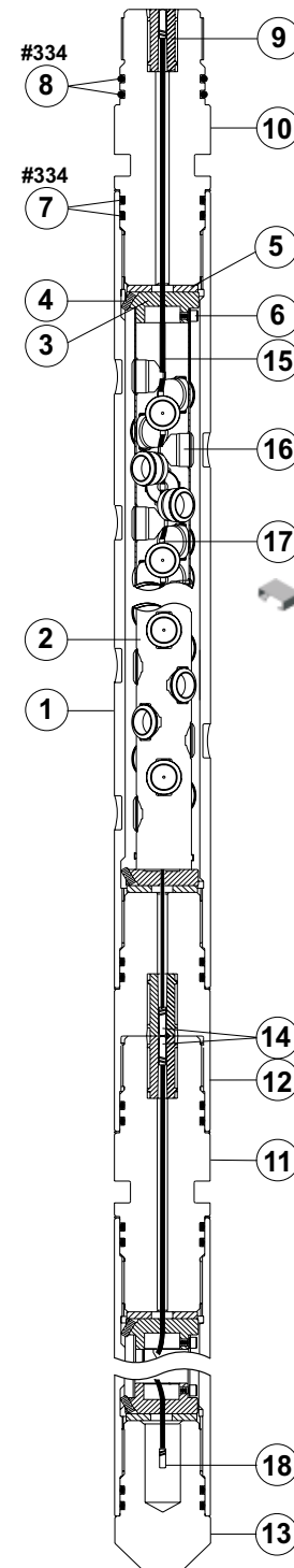
3 3/8-in. 12-spf OMNI™ VannGun™ System
