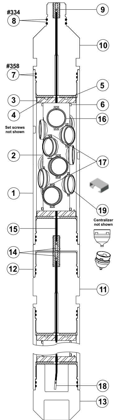
6 1/2-in. 12-spf 45°/135° VannGun™ System
