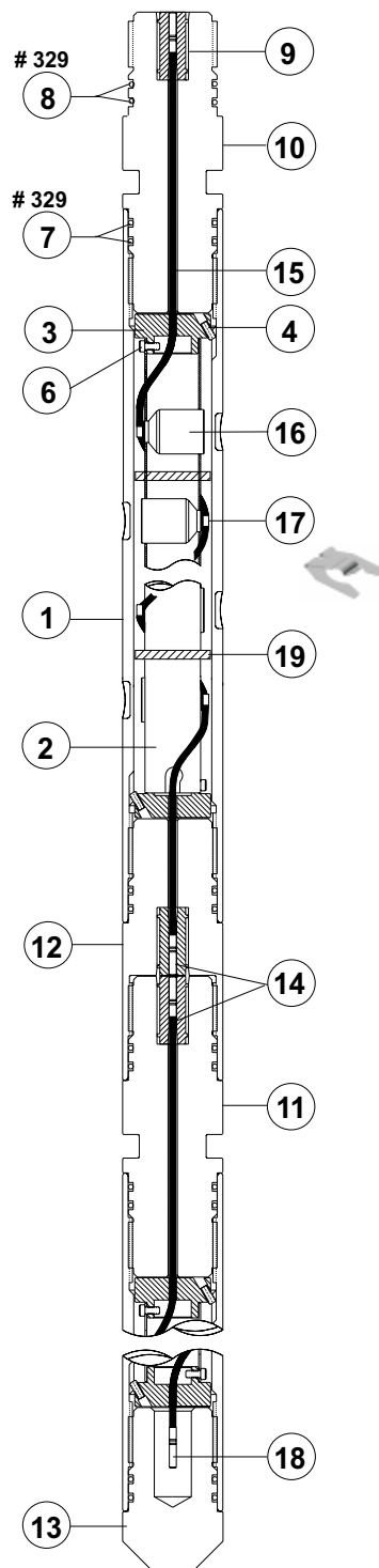
2 3/4 in. 4-spf 180° VannGun™ System
