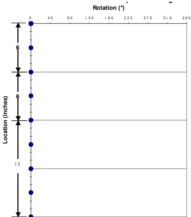
Shot Pattern for 2.5-in. 4-spf 0° Phasing
