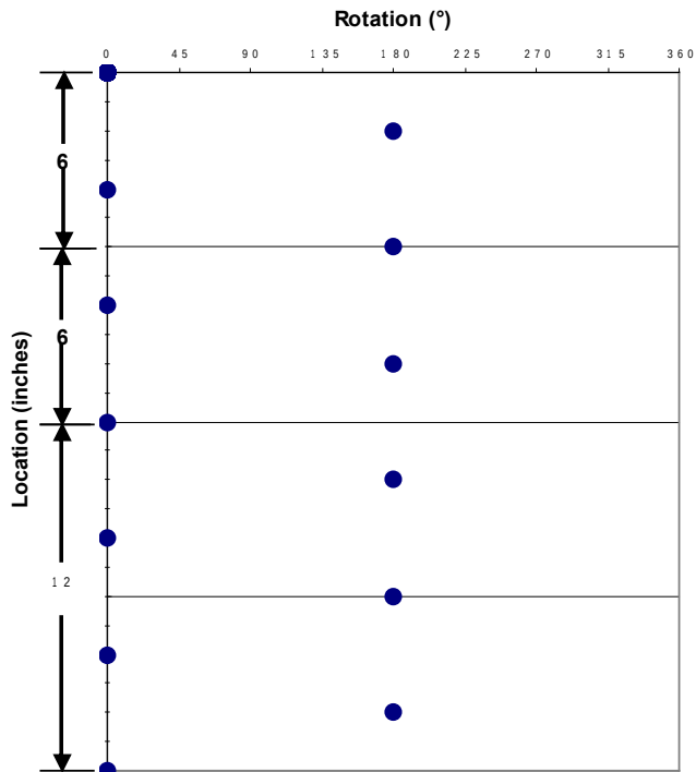
Shot Pattern for 1.5625-in. 6-spf 180° Phasing
