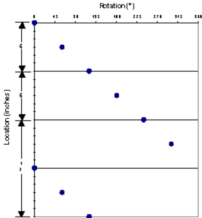
4-spf 60° Phasing
