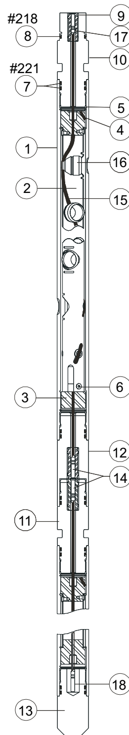
2-in. 4-spf 60° VannGun™ System
