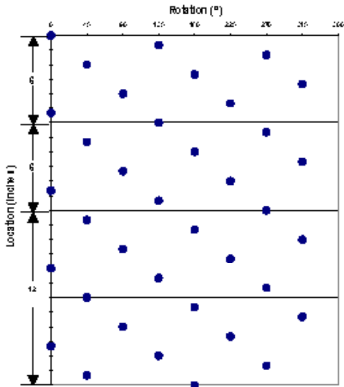
Shot Pattern for 4.625-in. 18-spf 45°/135° Phasing
