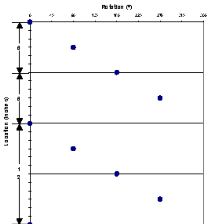
Shot Pattern for 4-in. 4-spf 90° Phasing
