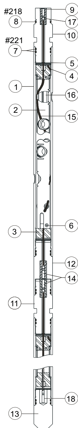
2-in. 6-spf 60° VannGun™ System
