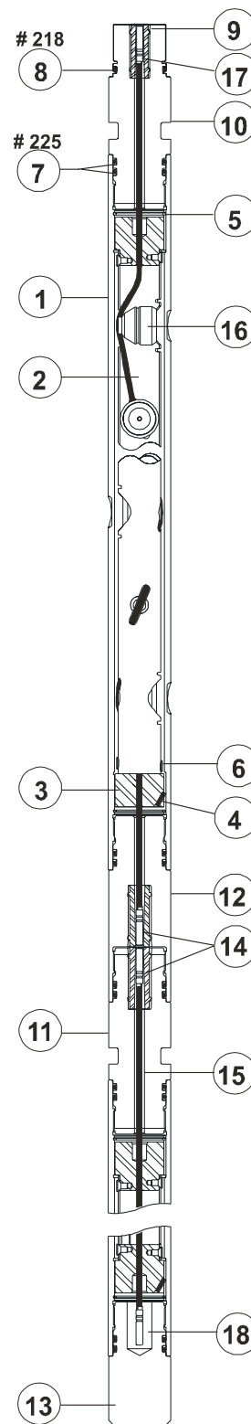
2 1/2-in. 6-spf 60° VannGun™ System
