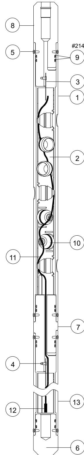
1 9/16-in. 6-spf 60° Slip-On Tube-Type
