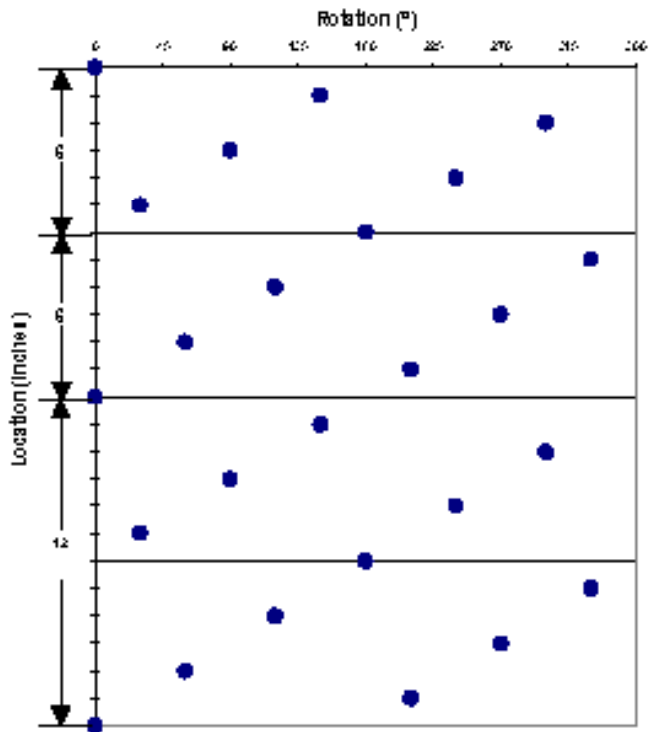
Shot Pattern for 4.75-in. 12-spf 30°/150° Phasing
