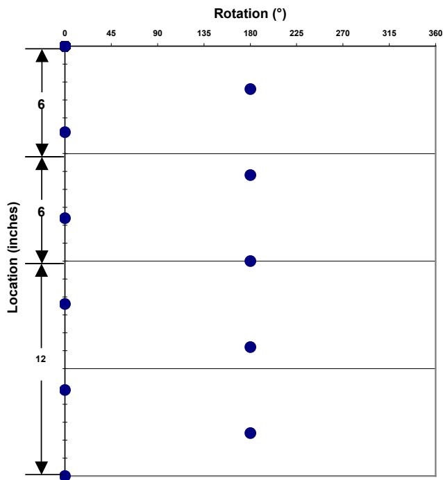
Shot Pattern for 2.75-in. 5-spf 180° Phasing
