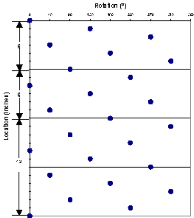
Shot Pattern for 6.5-in. 12-spf 45°/135° Phasing
