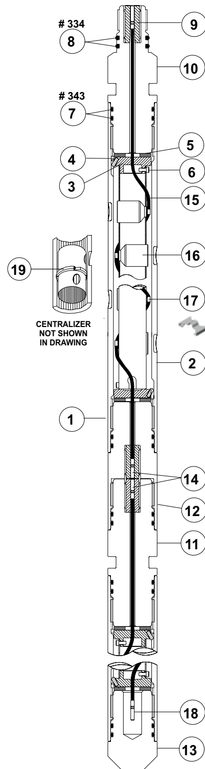
4 5/8-in. 4-spf 180° VannGun™ System
