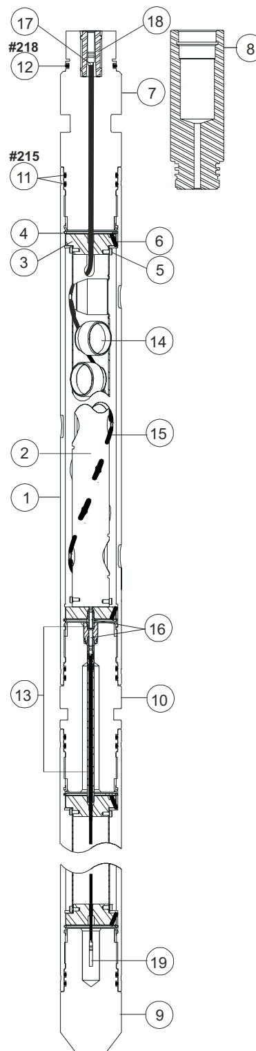
1 9/16-in. 6-spf 60° Scalloped System
