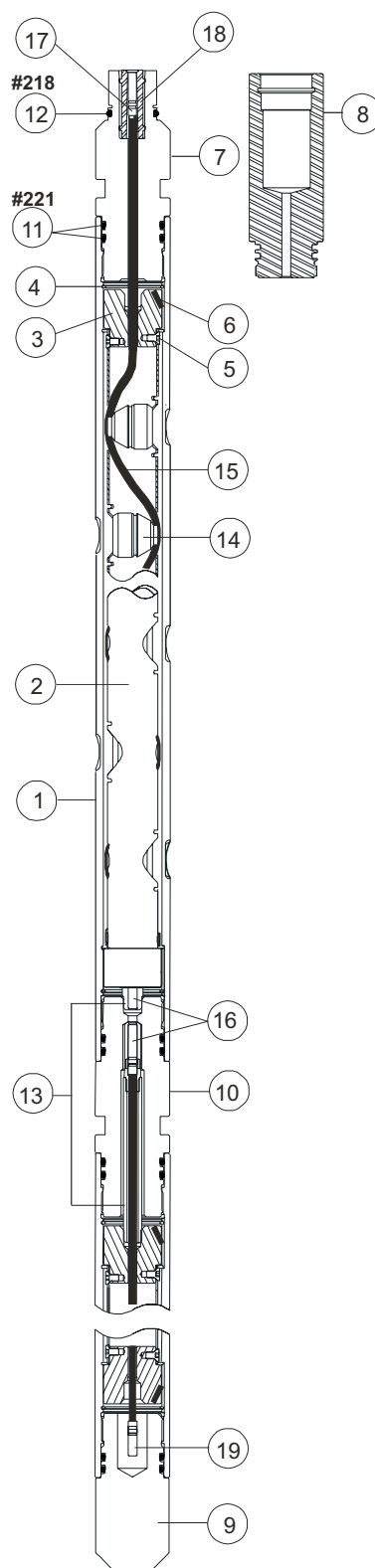
2-in. 4-spf 180° Scalloped System
