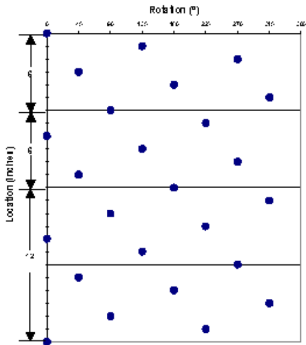
Shot Pattern for 5-in. 12-spf 45°/135° Phasing
