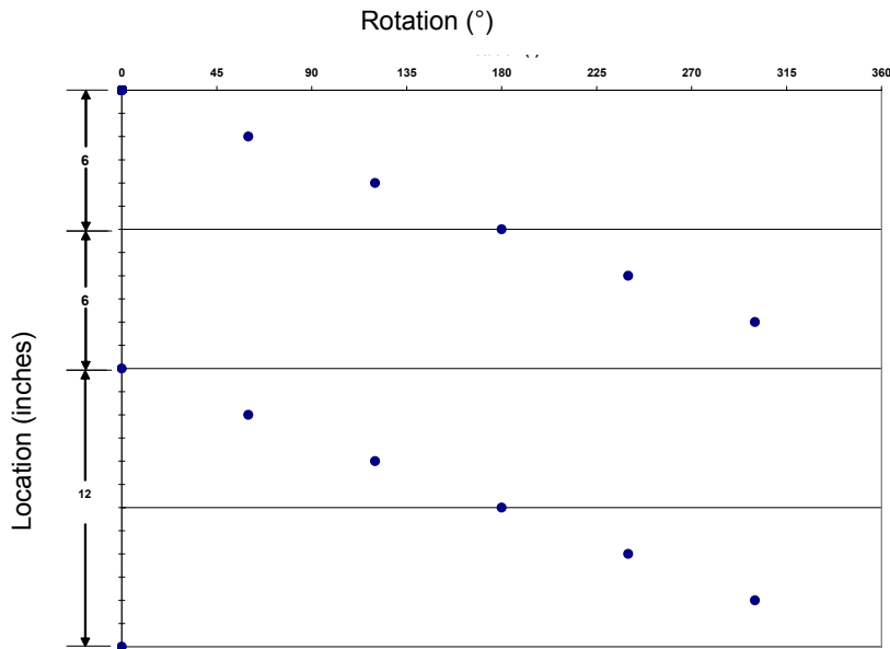
Shot Pattern for 2.875-in. 6-spf 60° Phasing
