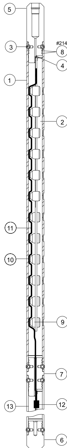
1 9/16-in. 4-spf 0° Slip-On Tubing Puncher
