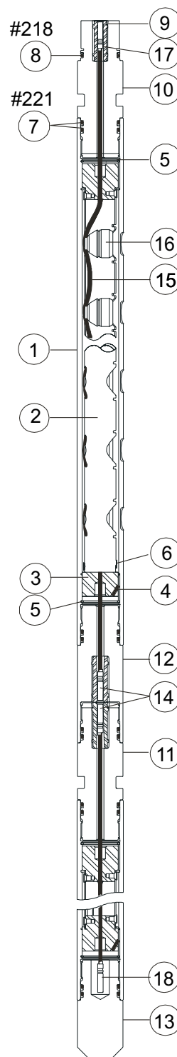
2-in. 4-spf 0° VannGun™ System
