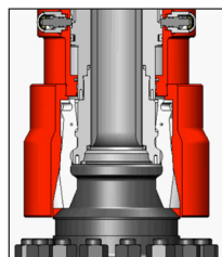
ExpressKinect™ Quick Latch secured.
