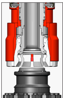
ExpressKinect™ Quick Latch opened.
