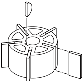
I MPA0801 Rotor, Vanes & Key Kit Code: 8993017711
