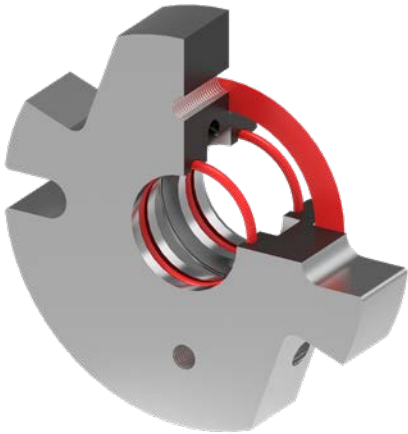
O-Pro® Cartridge Seal Cutaway
