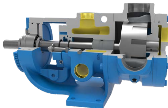
Standard-Jacketed Pump Cutaway – K1224A-ASP
