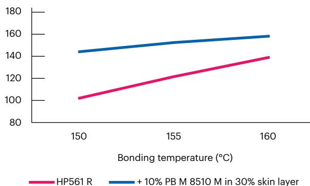
50 g/m 2 NW tensile strength MD (N/5cm)
