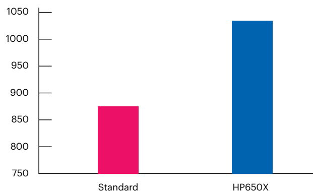
Hydrohead (mm) 20 g/m 2 fabrics
