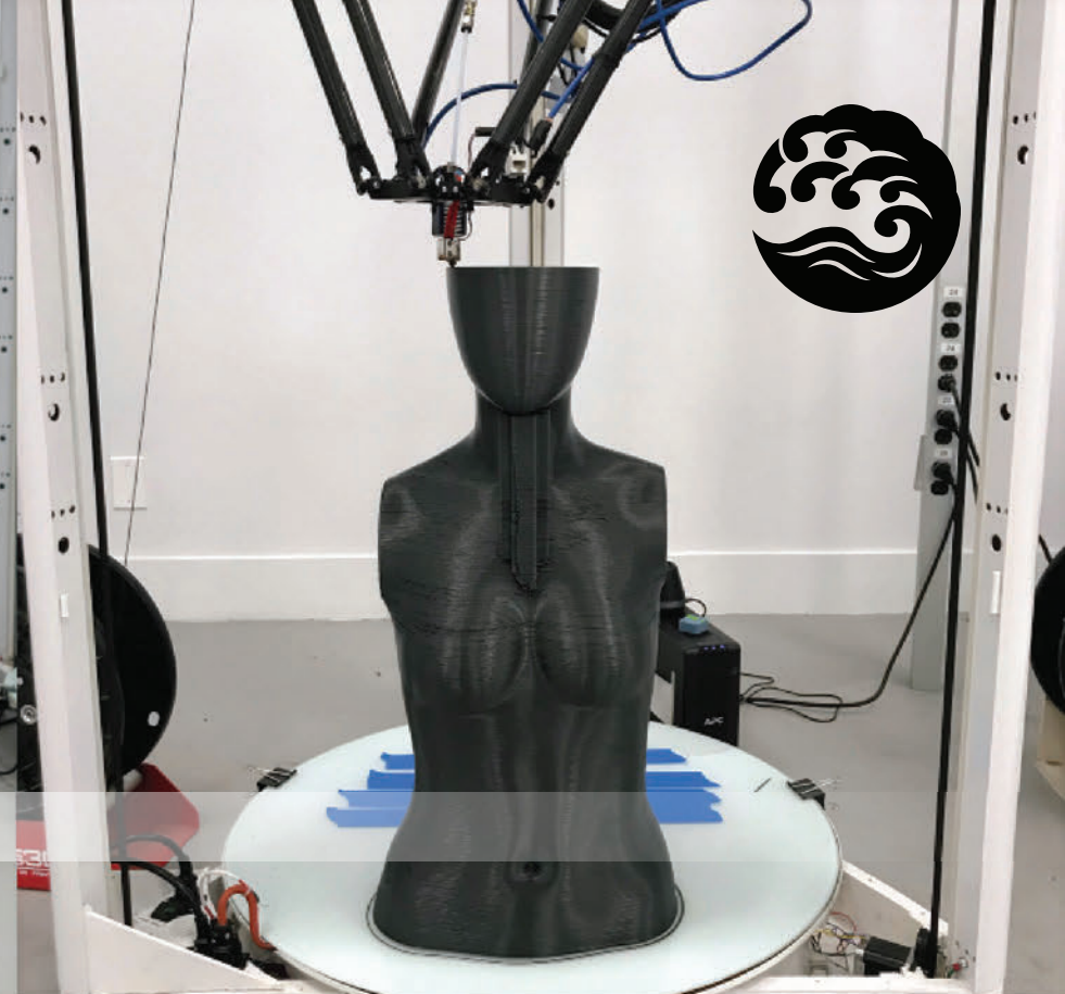
FDM PRINTING WITH ECO-T PLA
