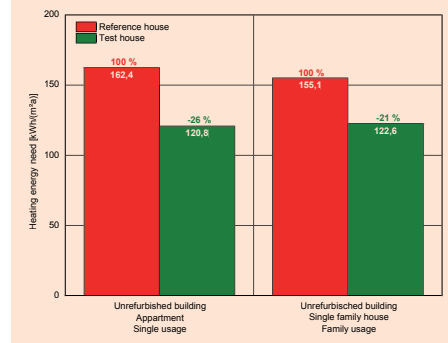
Fig. 1: Net heating energy savings for an unrefurbished apartment occupied by a single and for a single family house, occupied by a family.
