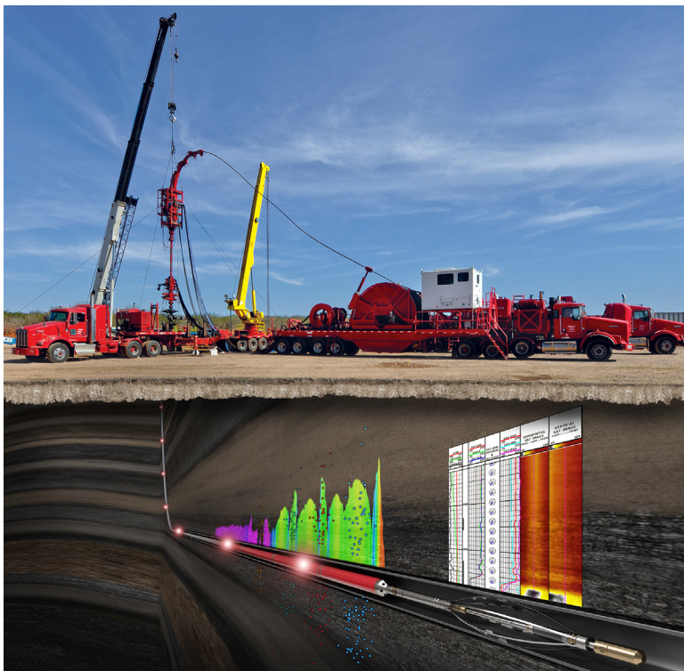
Example of a single trip deployment of distributed temperature sensing (DTS) and distributed acoustic sensing (DAS) and PLT with the SPECTRUM® Real-Time Hybrid Coiled Tubing Service for maximum production insight.
