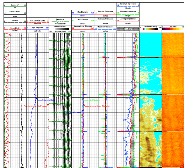
Cement evaluation and casing inspection logs from the BSAT™ and CAST-XR™ services are combined to provide the optimum zonal isolation and well integrity answers in high-thickness casings.
