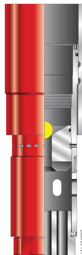
Landing collar latch type with catcher sub
